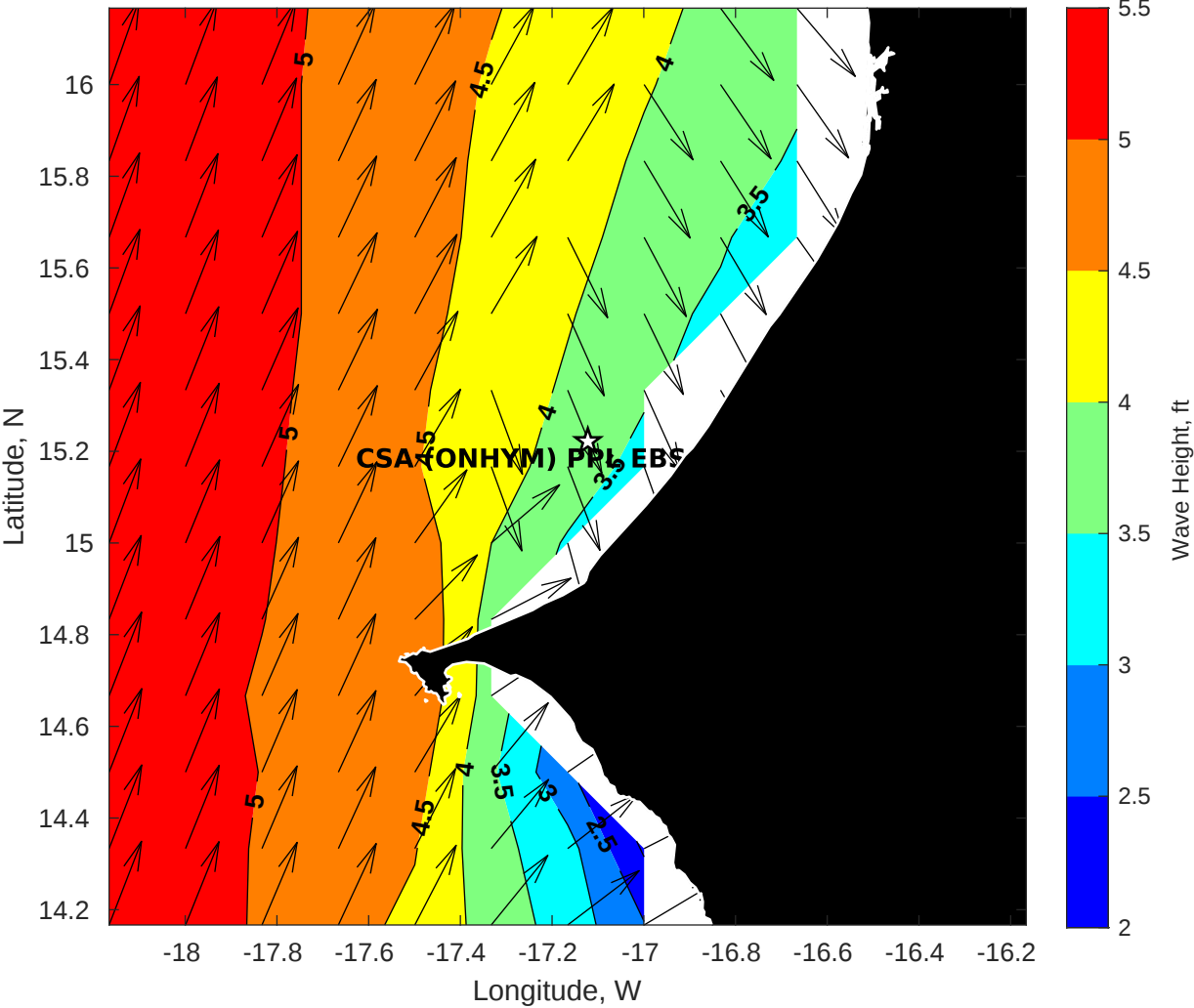
Wave Height (ft) for CSA (ONHYM) PPL EBS - Senegal at 05-Aug-2025 09:00:00
