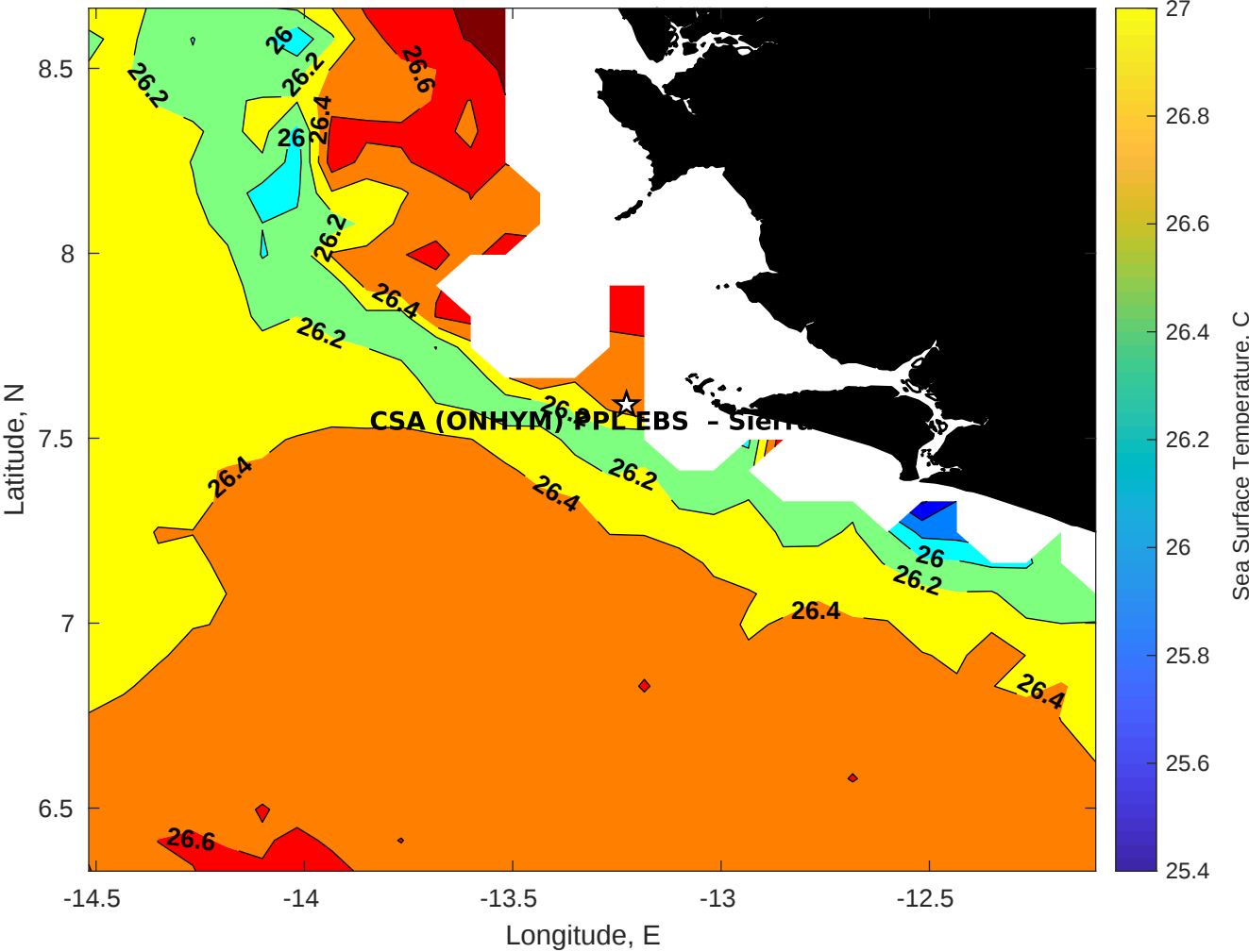
SST for CSA (ONHYM) PPL EBS - Sierra Leone at 04-Aug-2025 00:00:00
