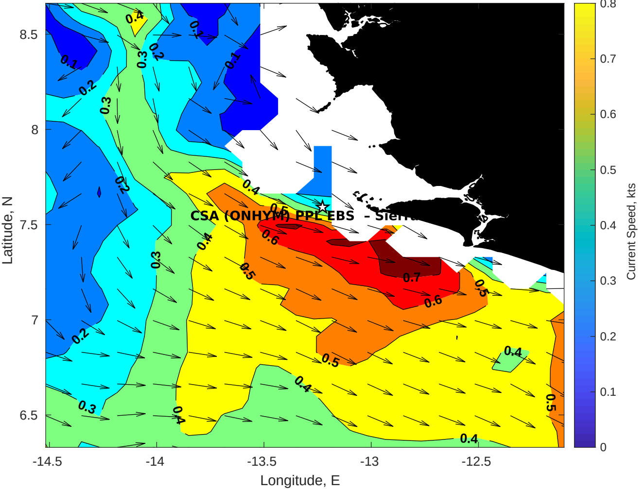
Surface Currents for CSA (ONHYM) PPL EBS - Sierra Leone at 04-Aug-2025 00:00:00
