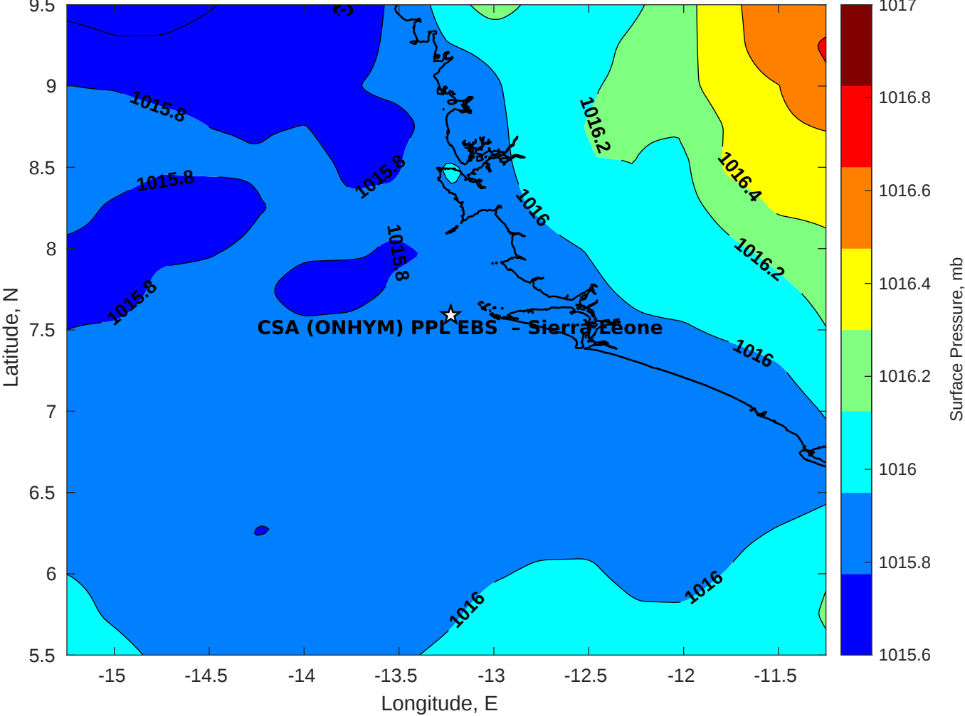
Surface Pressure (mb) for CSA (ONHYM) PPL EBS - Sierra Leone at 07-Aug-2025 00:00:00
