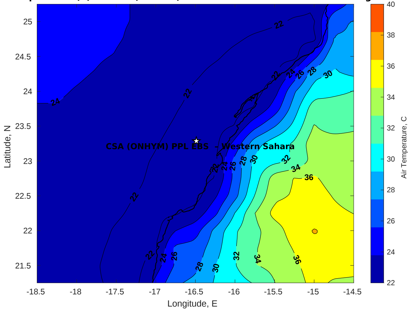
Air Temperature (C) for CSA (ONHYM) PPL EBS - Western Sahara at 05-Aug-2025
