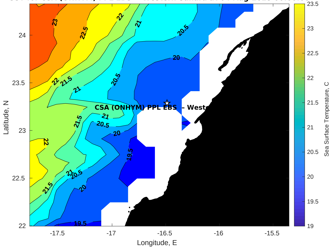
SST for CSA (ONHYM) PPL EBS - Western Sahara at 04-Aug-2025 00:00:00
