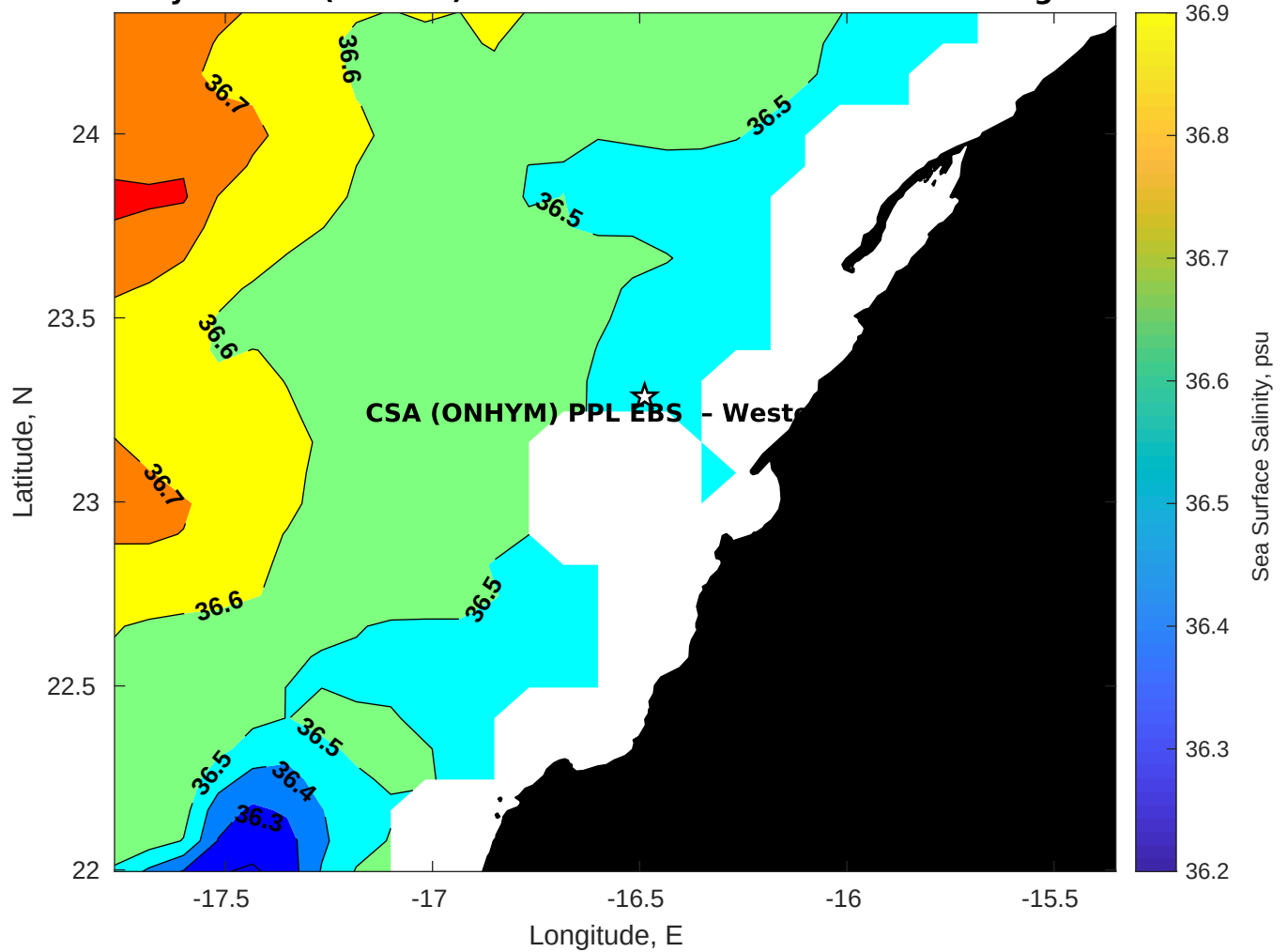
Surface Salinity for CSA (ONHYM) PPL EBS - Western Sahara at 04-Aug-2025 00:00:00
