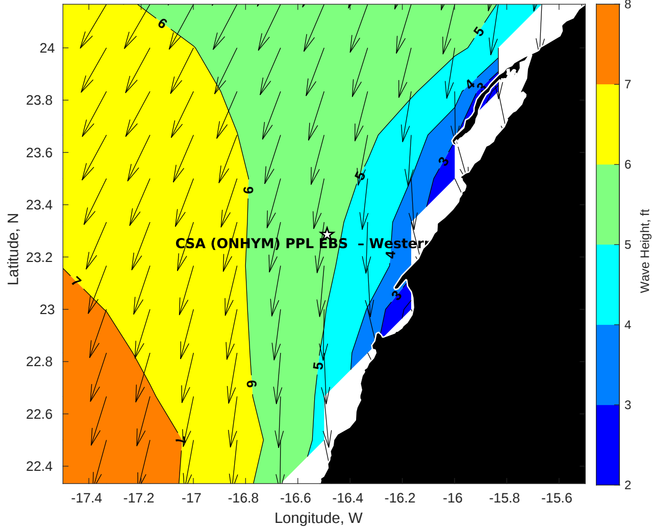
Wave Height (ft) for CSA (ONHYM) PPL EBS - Western Sahara at 05-Aug-2025 09:00:00
