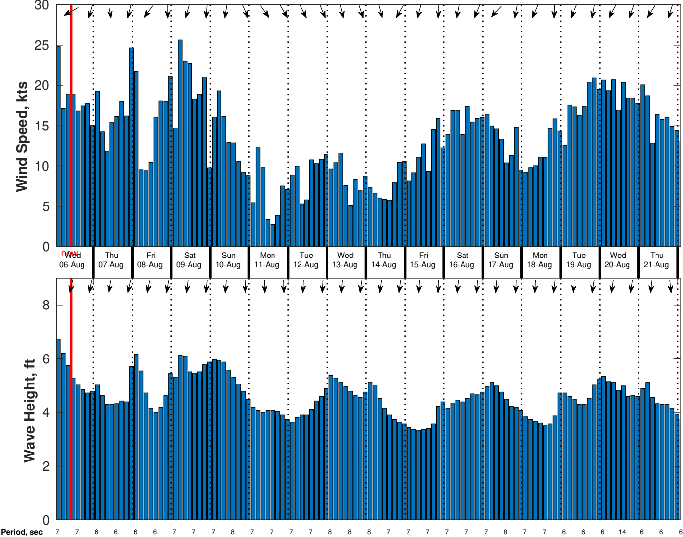
Wind & Wave Forecast for CSA (ONHYM) PPL EBS - Western Sahara from 05-Aug-2025 01:00:00 to 21-Aug-2025 01:00:00
