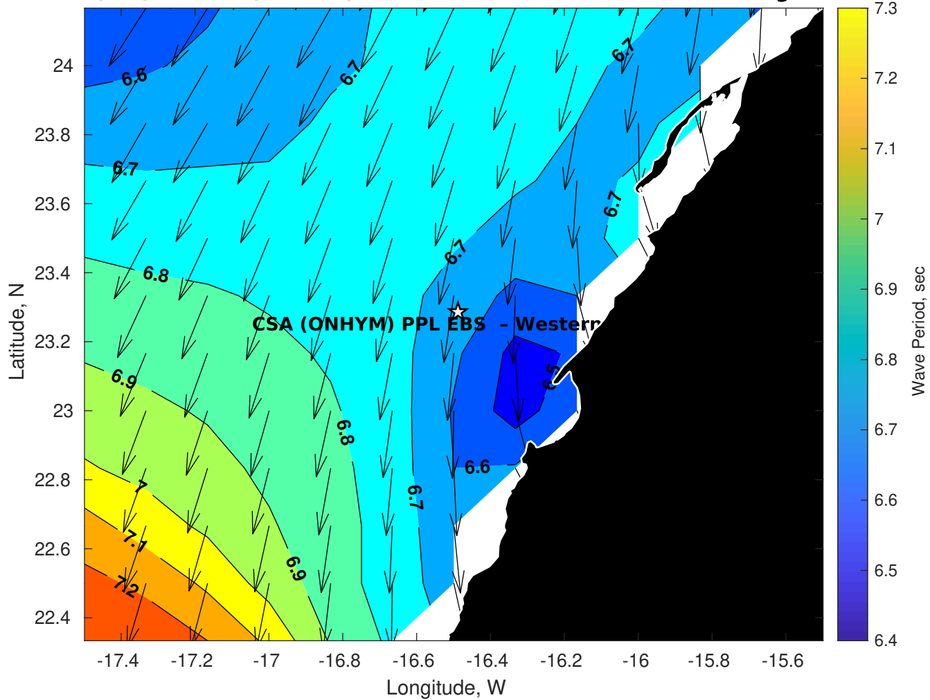
Wave Period (sec) for CSA (ONHYM) PPL EBS - Western Sahara at 05-Aug-2025 09:00:00
