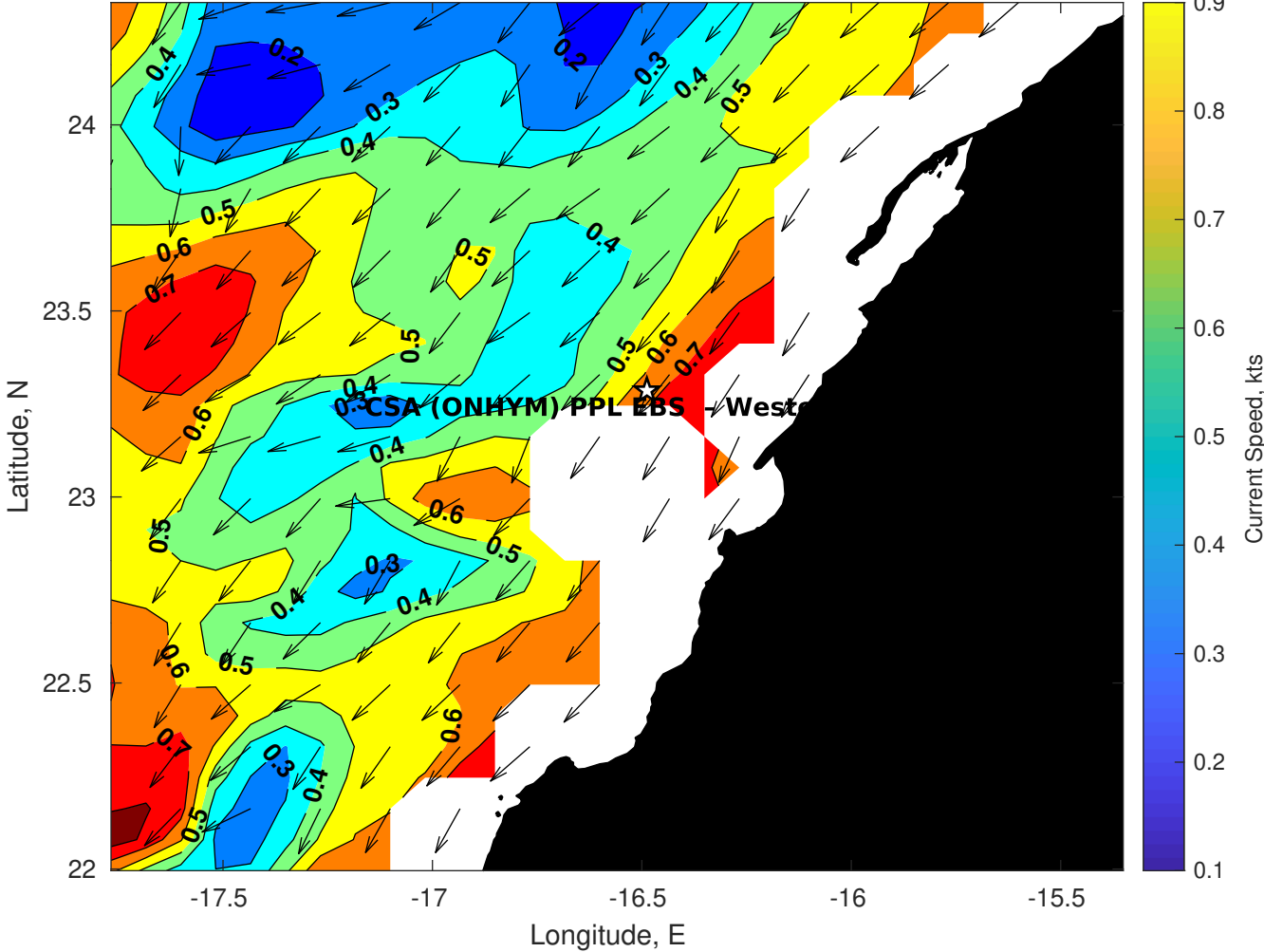
Surface Currents for CSA (ONHYM) PPL EBS - Western Sahara at 04-Aug-2025 00:00:00
