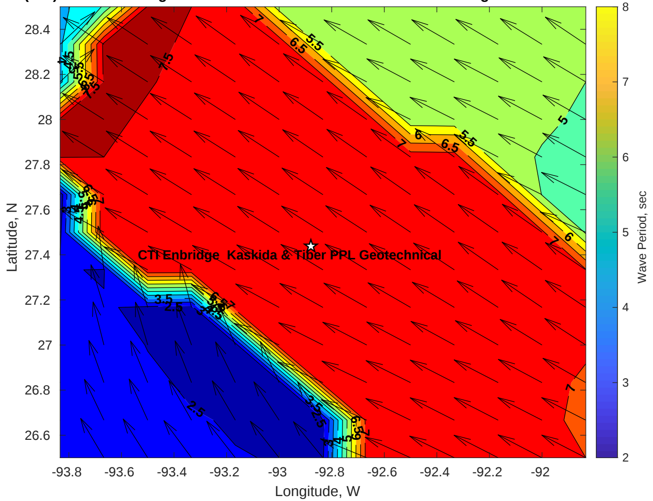
Wave Period (sec) for CTI Enbridge Kaskida & Tiber PPL Geotechnical at 05-Aug-2025 09:00:00
