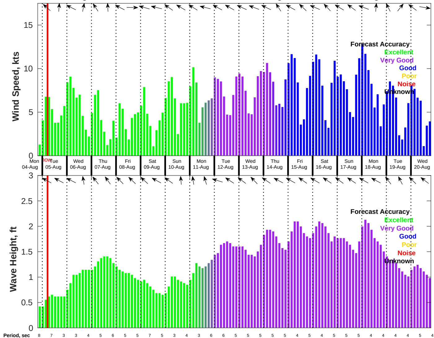
Wind & Wave Forecast for CTI Enbridge Kaskida & Tiber PPL Geotechnical from 04-Aug-2025 20:00:00 to 20-Aug-2025 20:00:00
