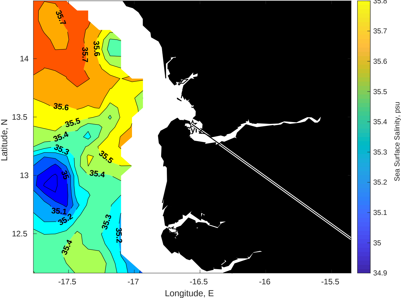
Surface Salinity for Gyre at 04-Aug-2025 00:00:00
