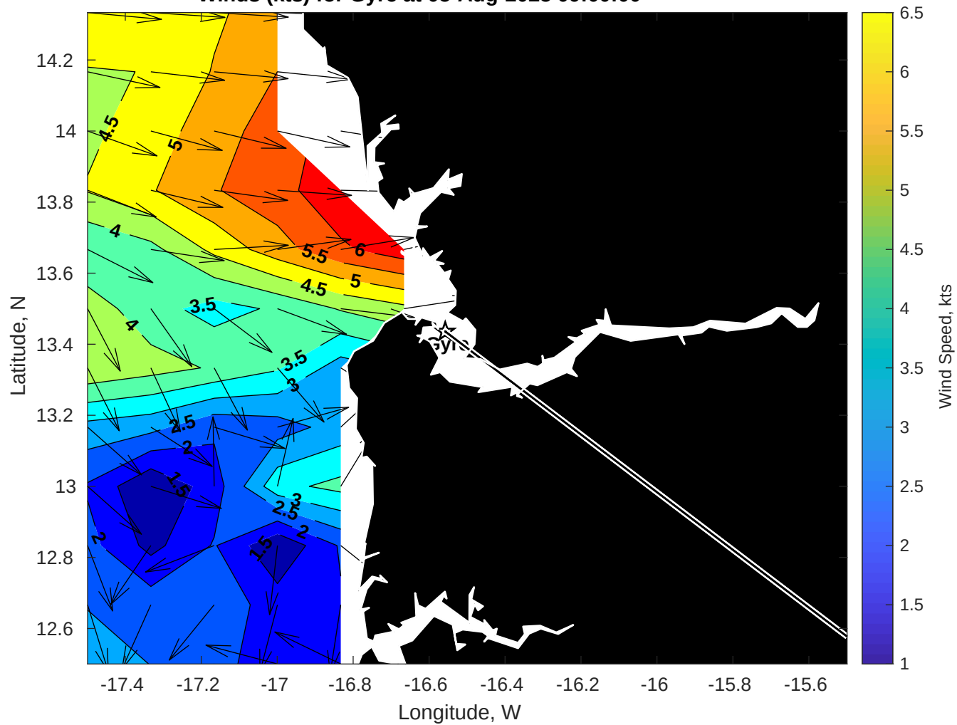
Winds (kts) for Gyre at 05-Aug-2025 09:00:00
