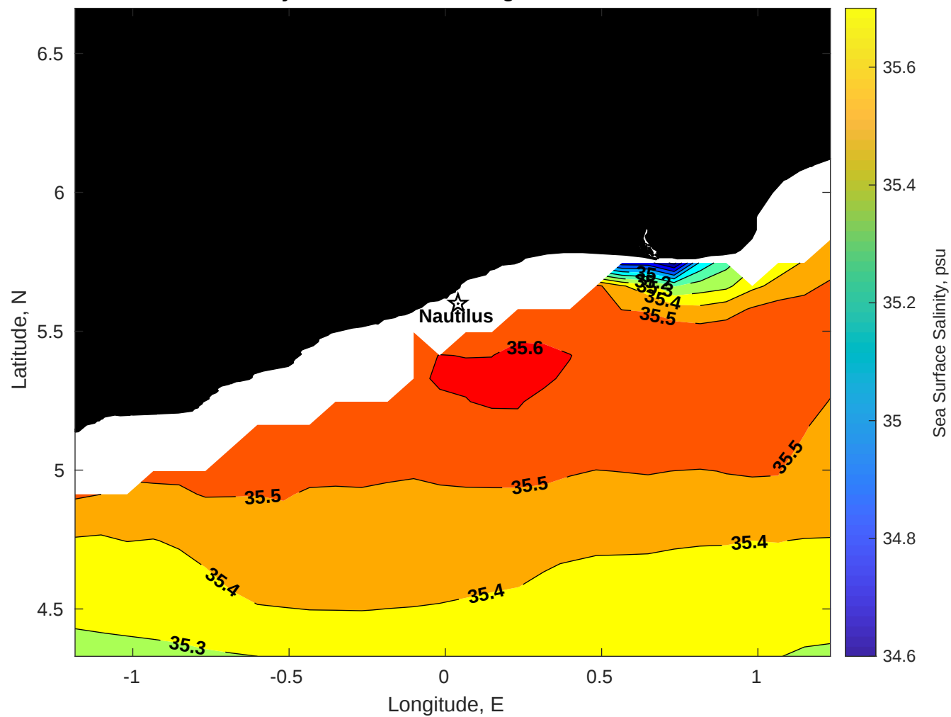
Surface Salinity for Nautilus at 04-Aug-2025 00:00:00
