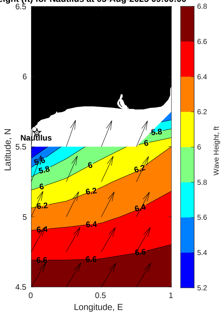
Wave Height (ft) for Nautilus at 05-Aug-2025 09:00:00
