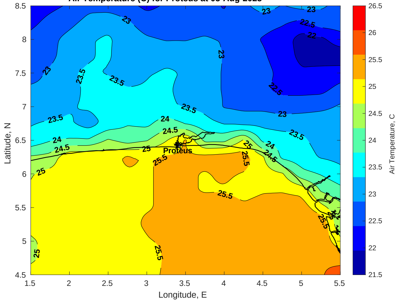
Air Temperature (C) for Proteus at 05-Aug-2025
