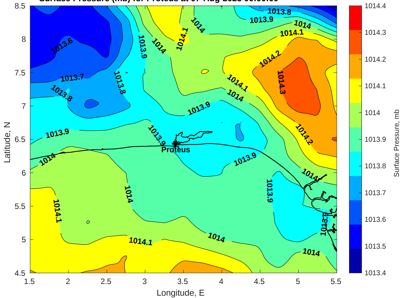
Surface Pressure (mb) for Proteus at 07-Aug-2025 00:00:00
