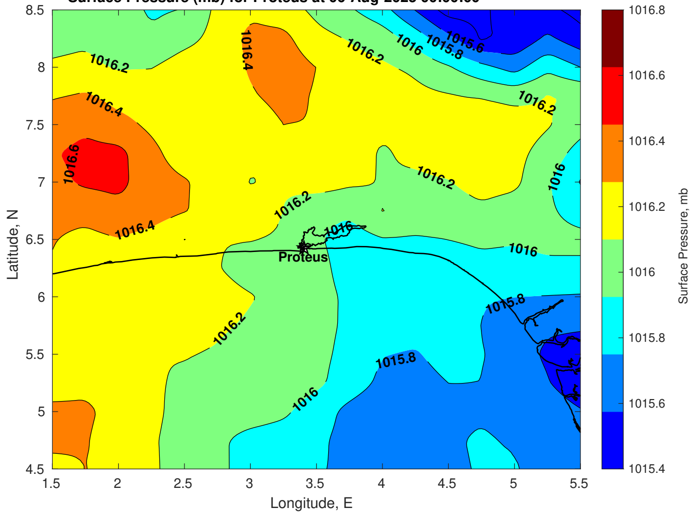
Surface Pressure (mb) for Proteus at 06-Aug-2025 00:00:00
