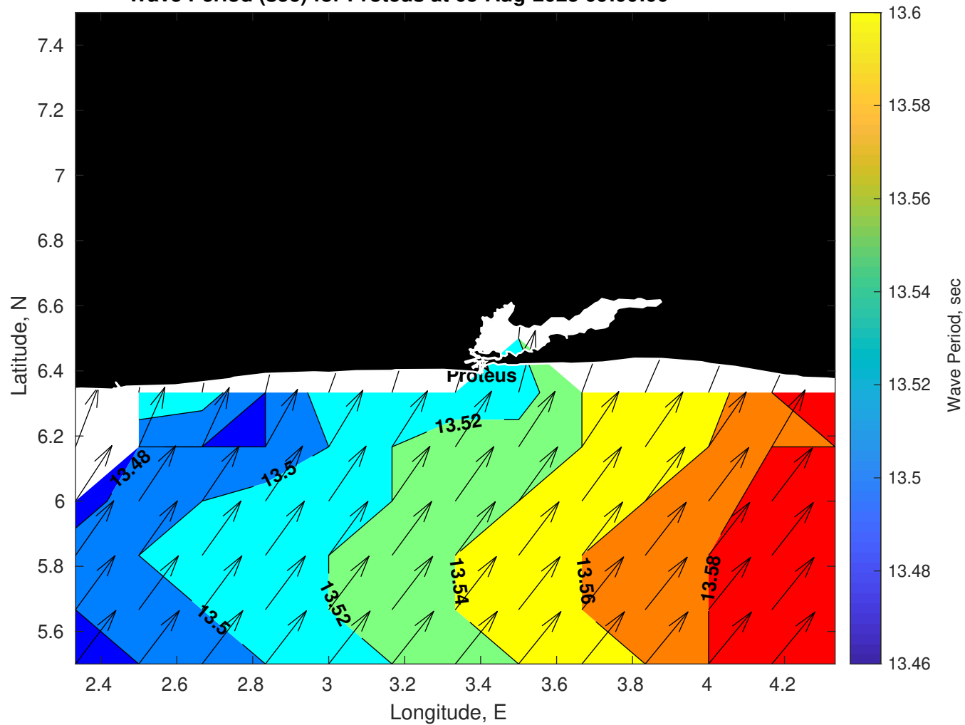
Wave Period (sec) for Proteus at 05-Aug-2025 09:00:00
