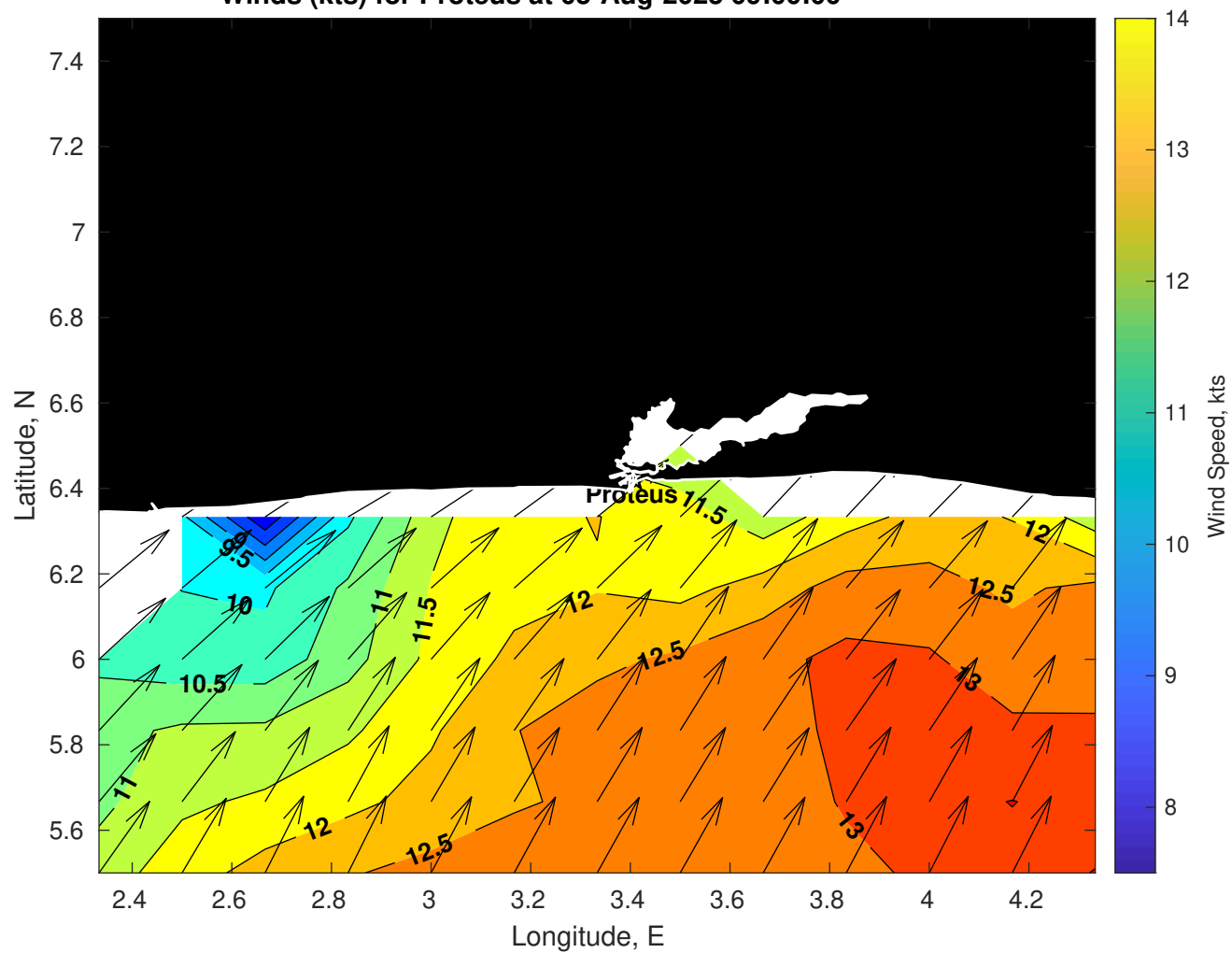
Winds (kts) for Proteus at 05-Aug-2025 09:00:00
