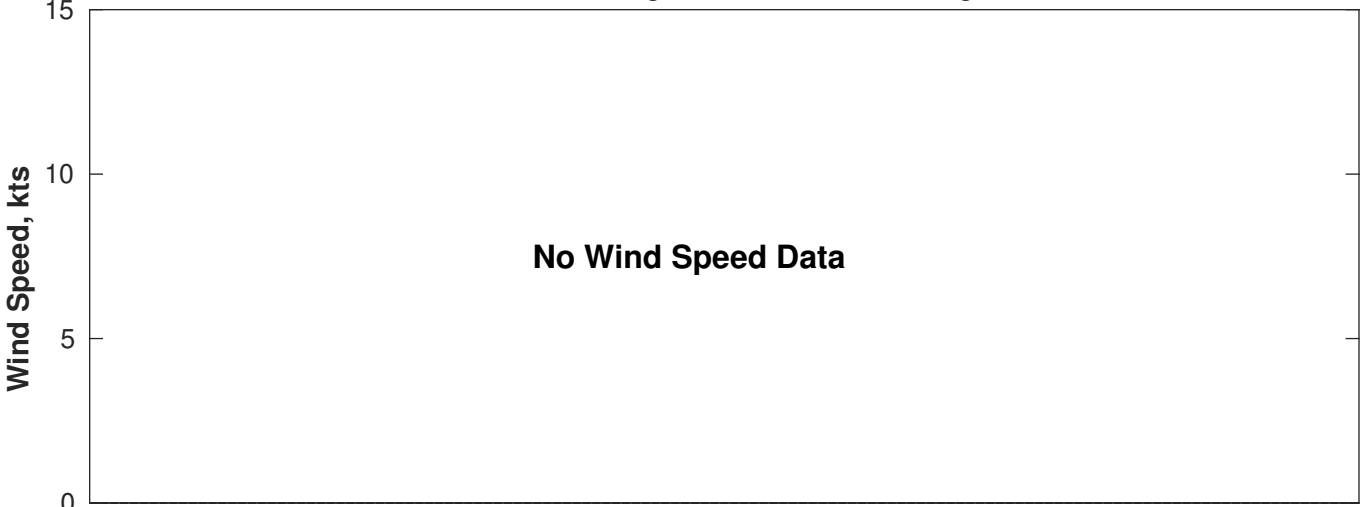
Wind & Wave Forecast for Proteus from 05-Aug-2025 01:00:00 to 21-Aug-2025 01:00:00
