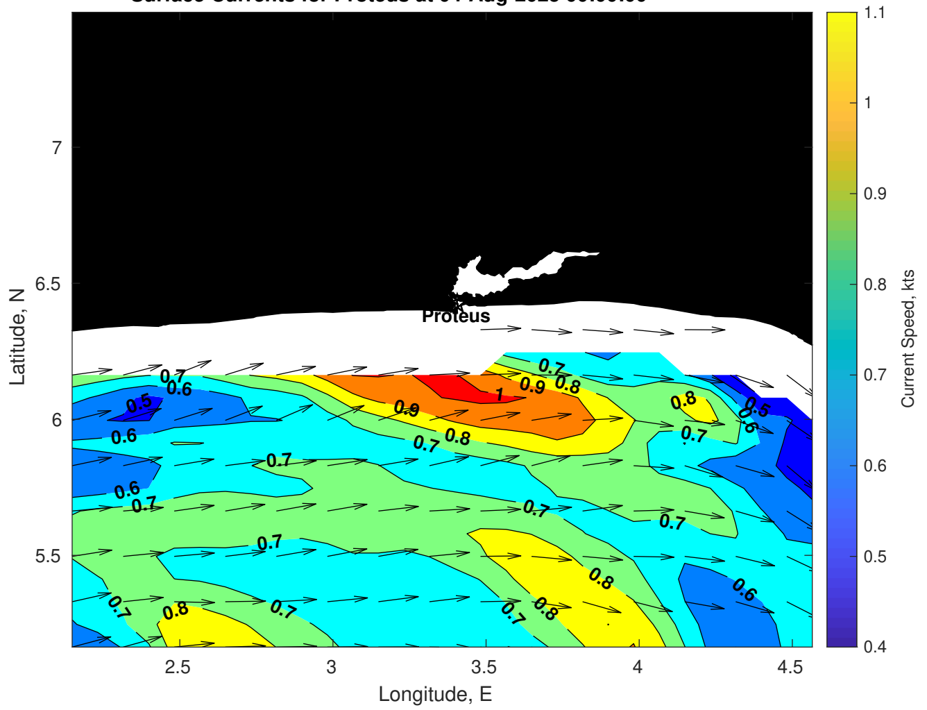
Surface Currents for Proteus at 04-Aug-2025 00:00:00
