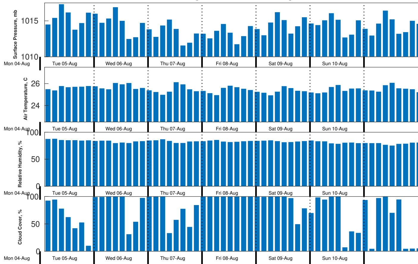
Met Forecast for Proteus from 05-Aug-2025 00:00:00 to 12-Aug-2025 00:00:00
