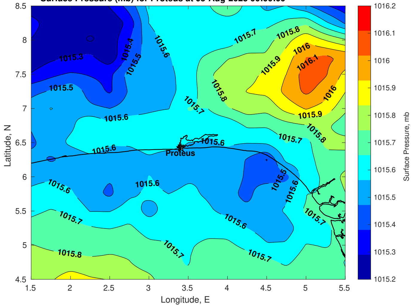
Surface Pressure (mb) for Proteus at 05-Aug-2025 00:00:00
