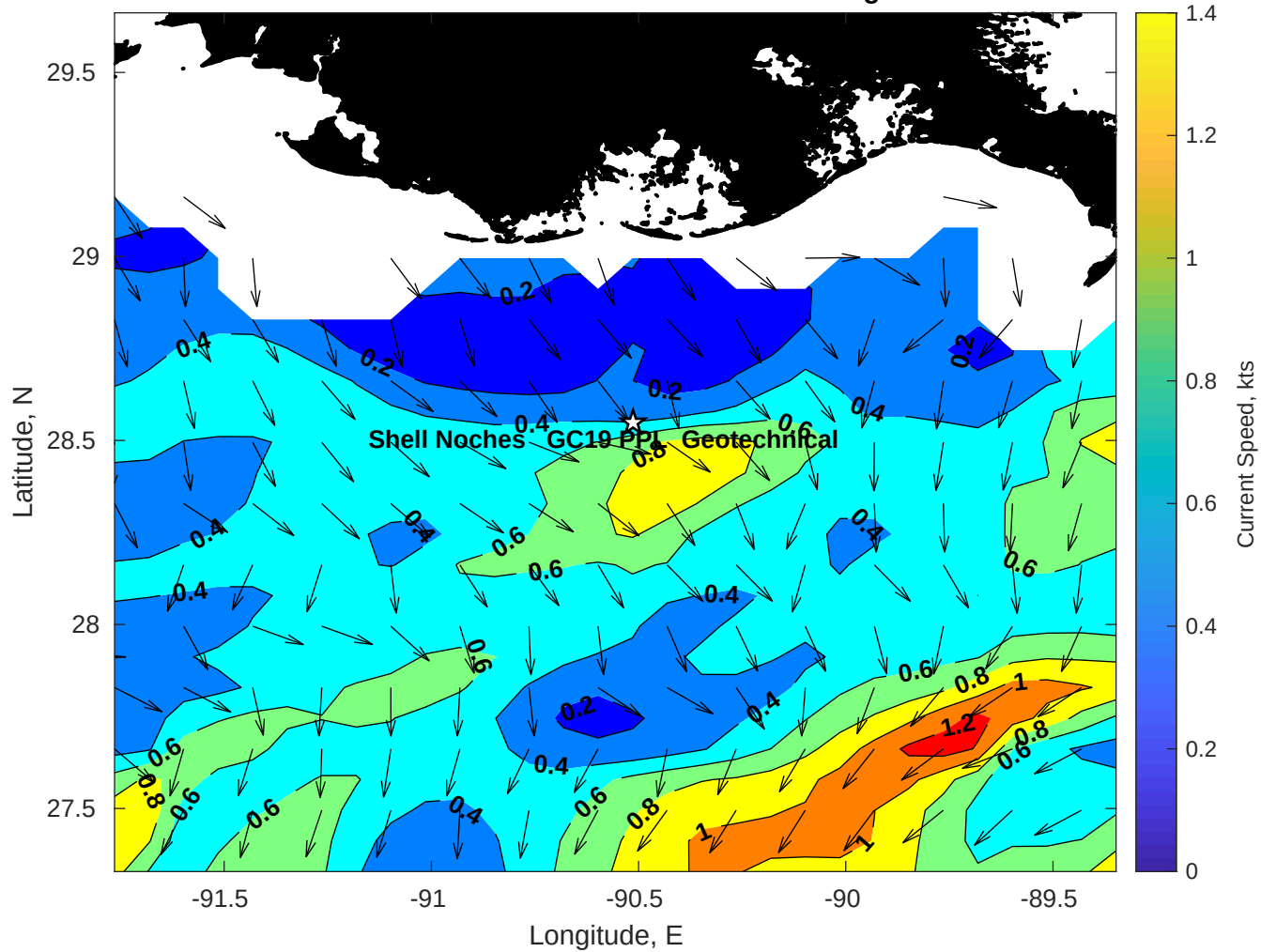
Surface Currents for Shell Noches GC19 PPL Geotechnical at 04-Aug-2025 00:00:00
