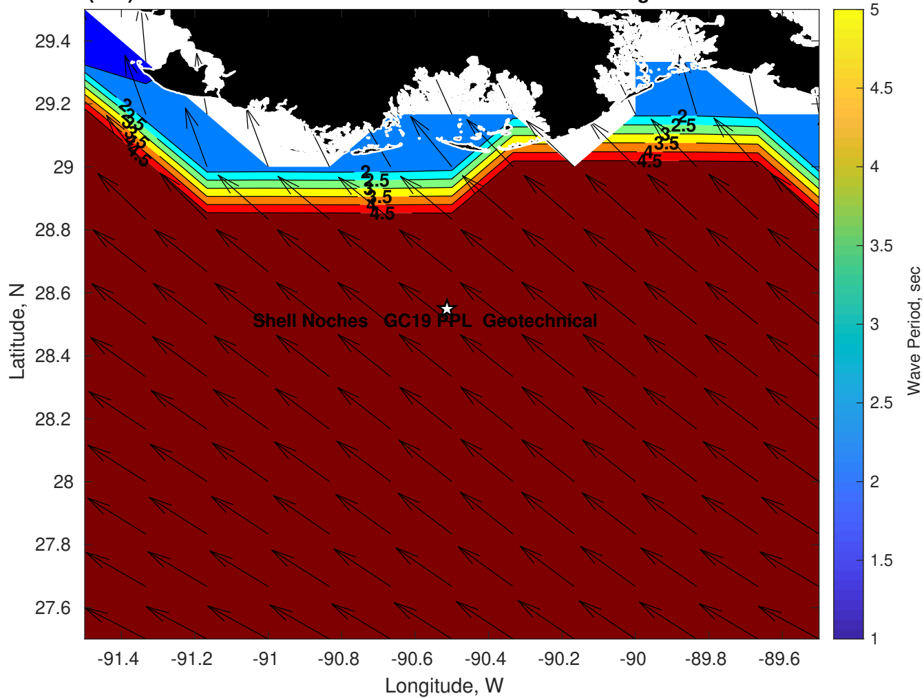
Wave Period (sec) for Shell Noches GC19 PPL Geotechnical at 05-Aug-2025 09:00:00
