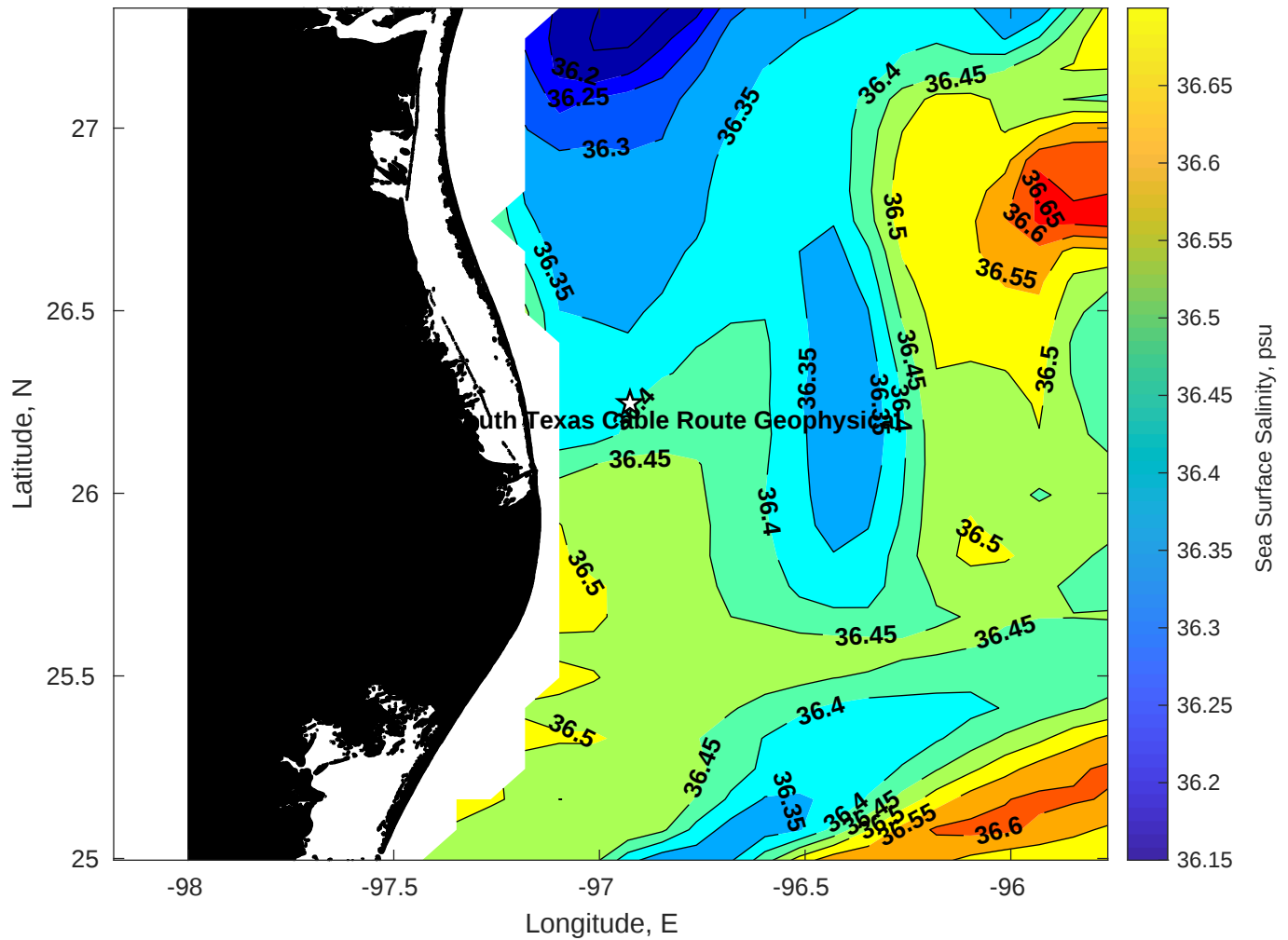
Surface Salinity for Tampnet P2378 South Texas Cable Route Geophysical at 04-Aug-2025 00:00:00
