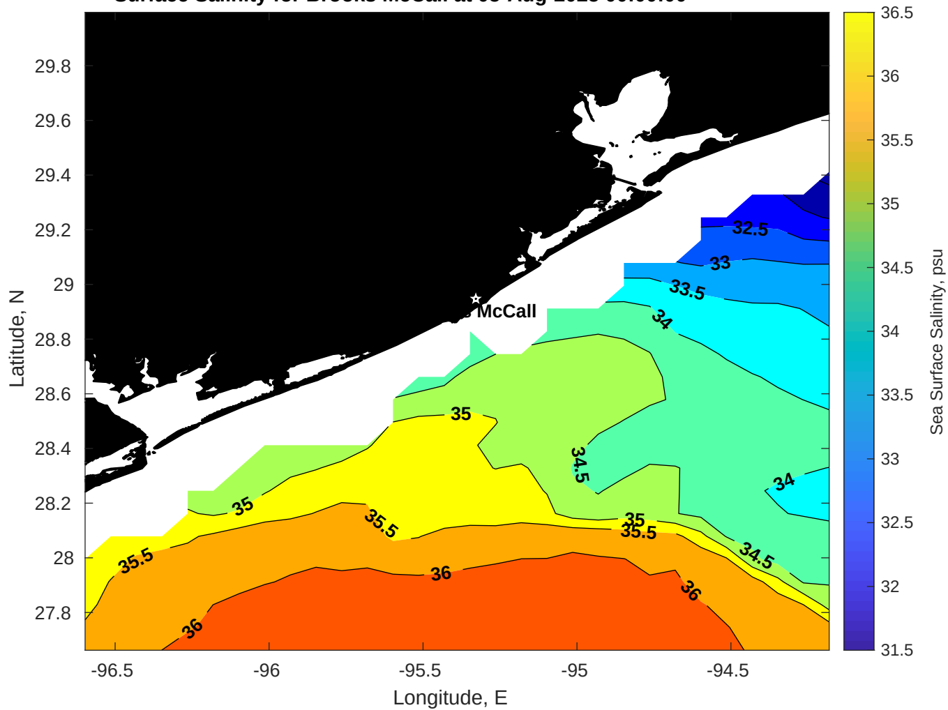
Surface Salinity for Brooks McCall at 05-Aug-2025 00:00:00
