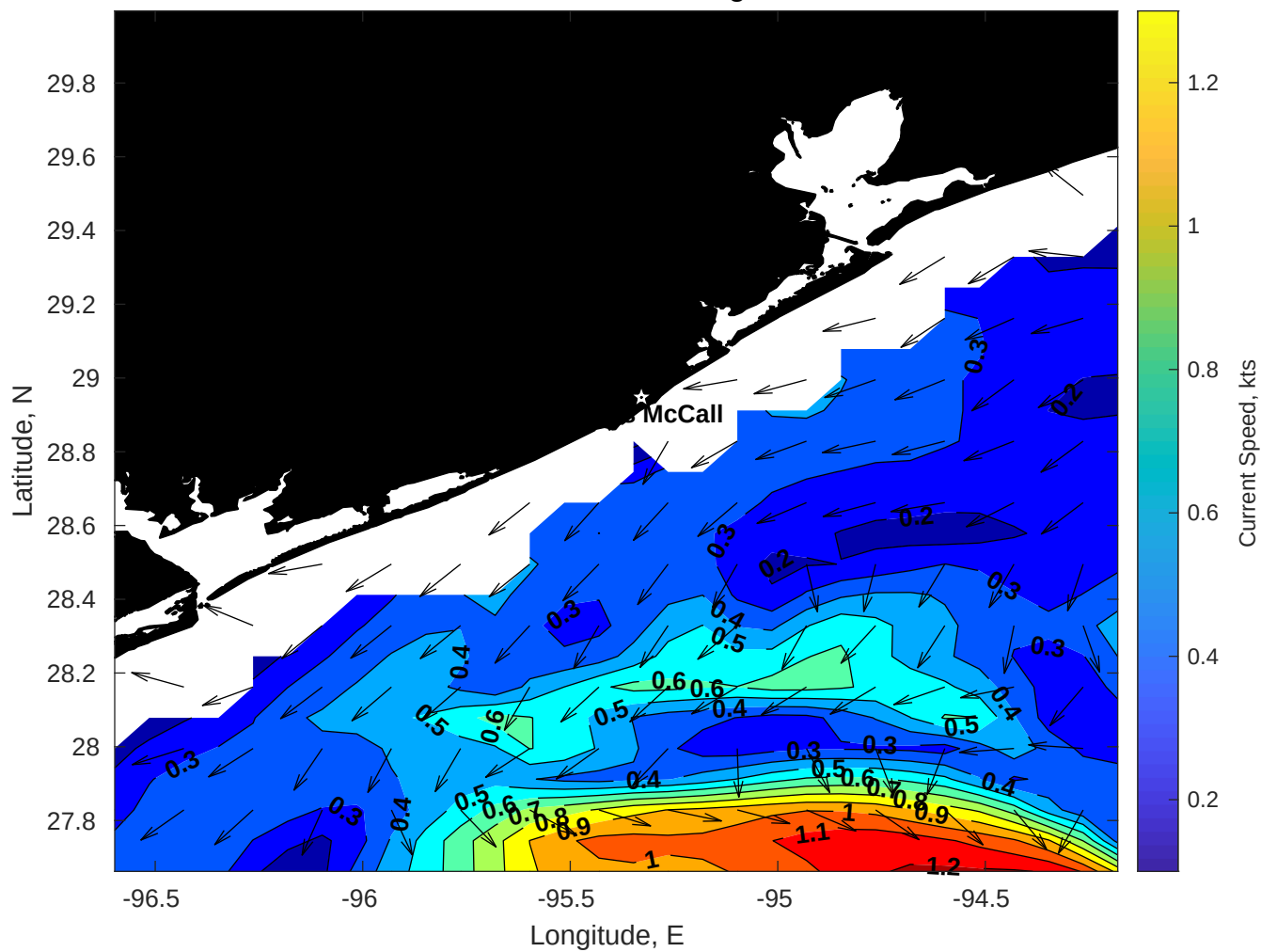
Surface Currents for Brooks McCall at 05-Aug-2025 00:00:00
