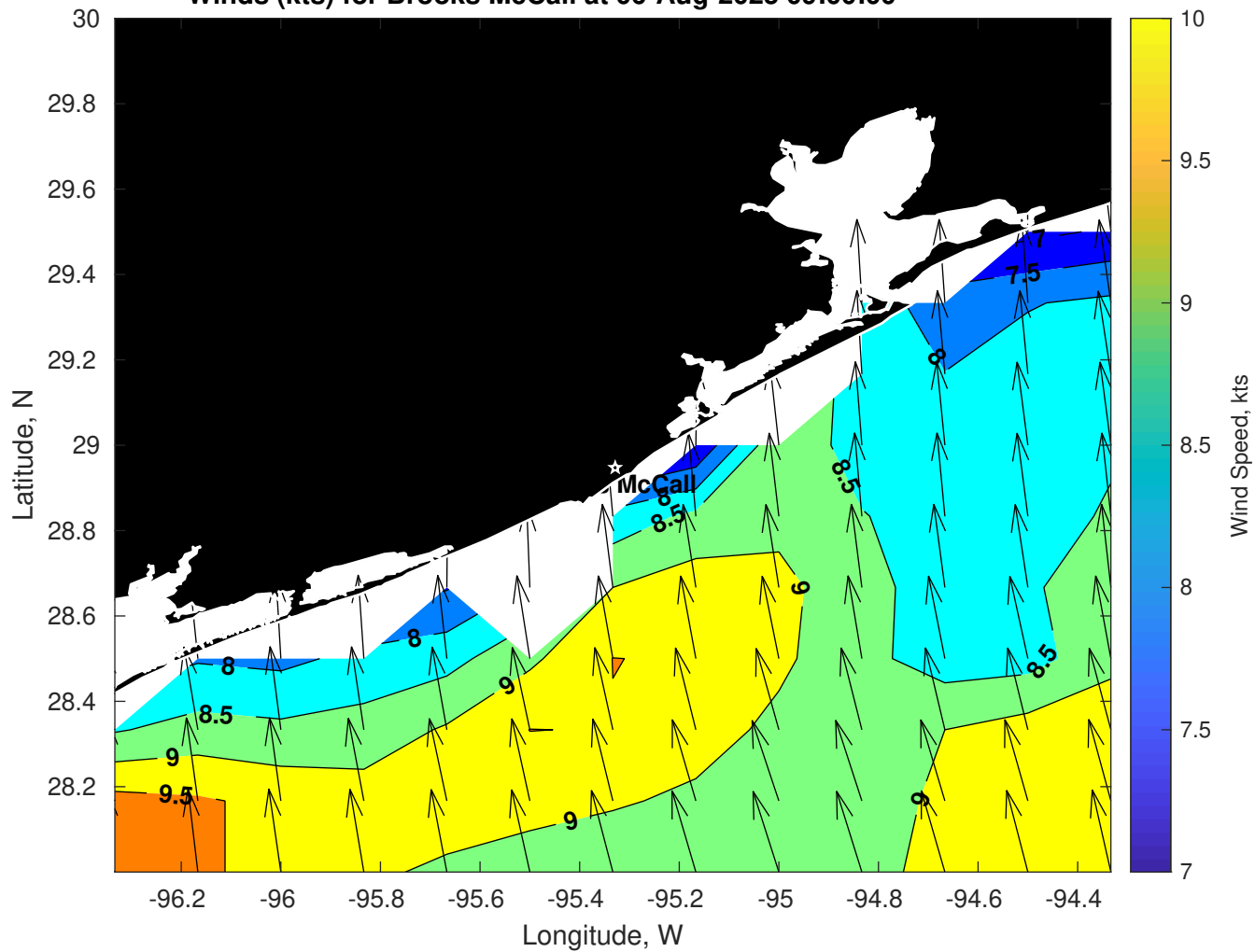
Winds (kts) for Brooks McCall at 06-Aug-2025 09:00:00
