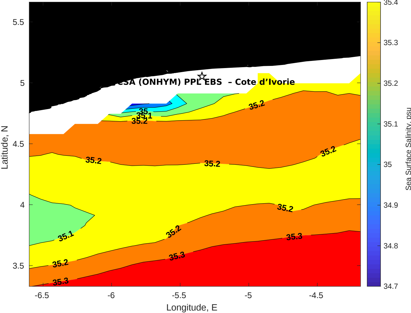
Surface Salinity for CSA (ONHYM) PPL EBS - Cote d'Ivoire at 05-Aug-2025 00:00:00
