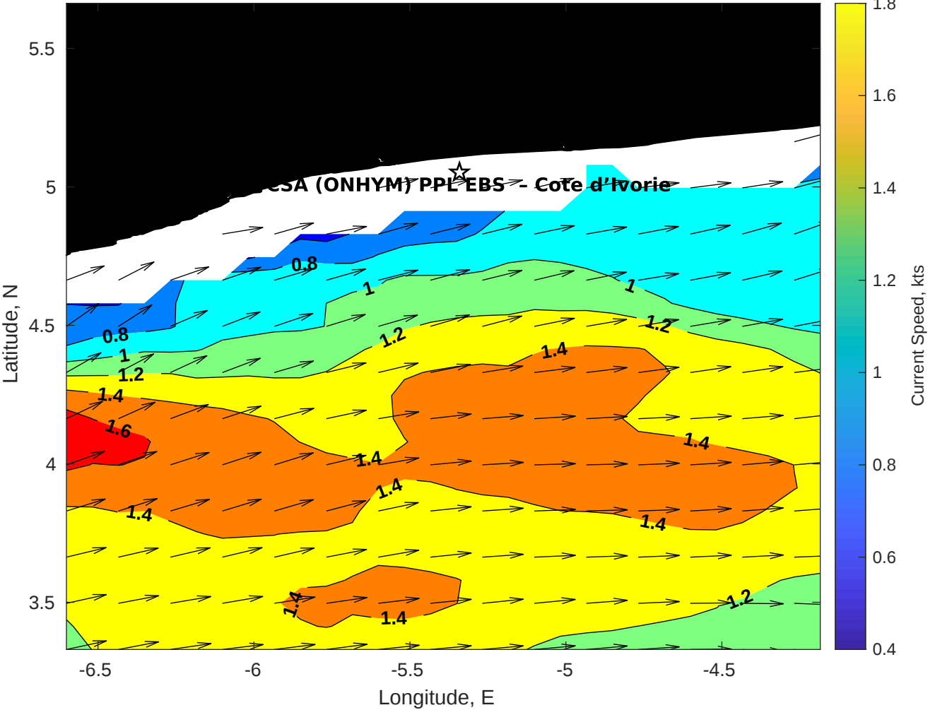
Surface Currents for CSA (ONHYM) PPL EBS - Cote d'Ivoire at 05-Aug-2025 00:00:00
