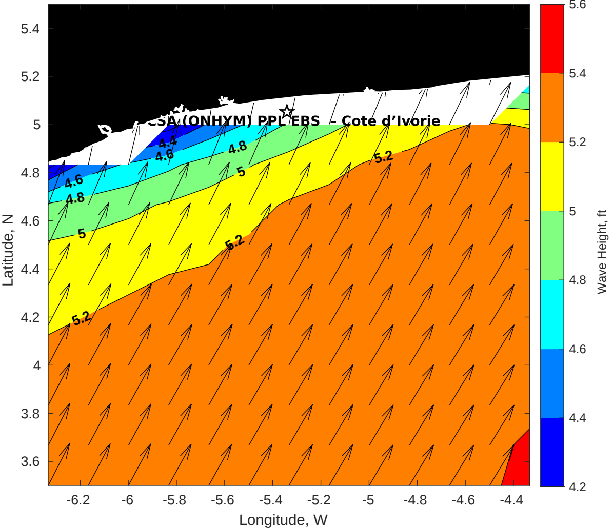
Wave Height (ft) for CSA (ONHYM) PPL EBS - Cote d'Ivoire at 06-Aug-2025 09:00:00
