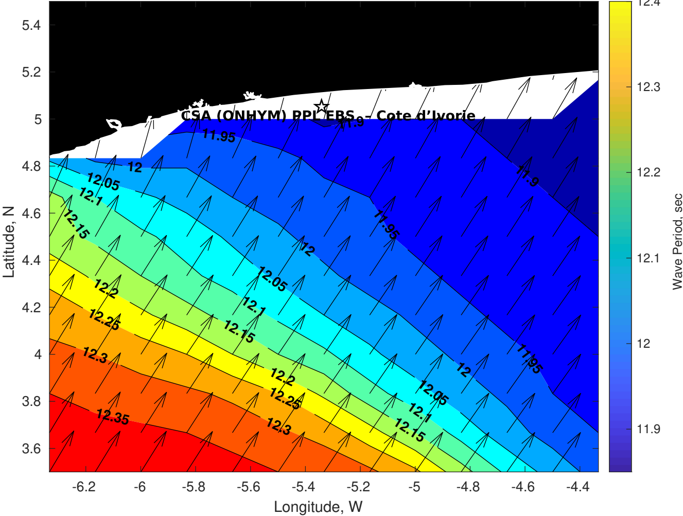
Wave Period (sec) for CSA (ONHYM) PPL EBS - Cote d'Ivoire at 06-Aug-2025 09:00:00
