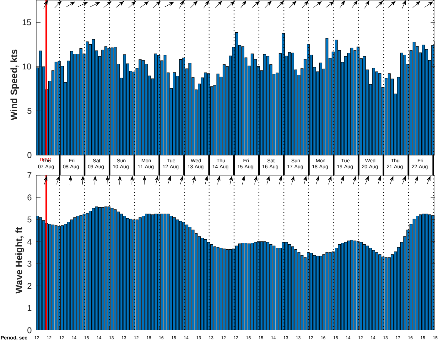
Wind & Wave Forecast for CSA (ONHYM) PPL EBS - Cote d'Ivoire from 06-Aug-2025 01:00:00 to 22-Aug-2025 01:00:00
