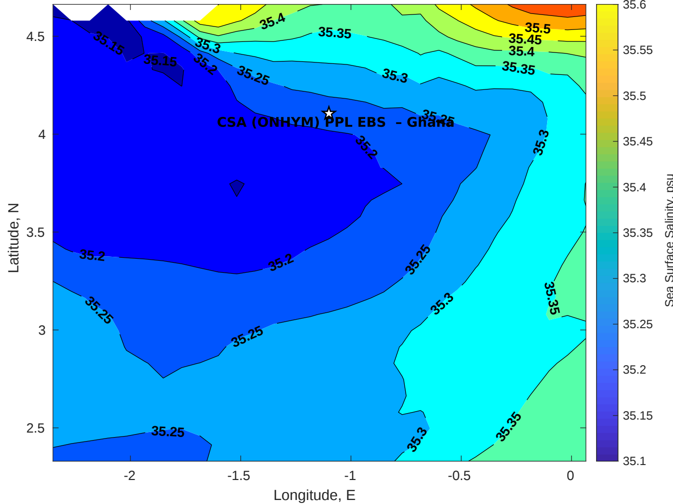
Surface Salinity for CSA (ONHYM) PPL EBS - Ghana at 05-Aug-2025 00:00:00
