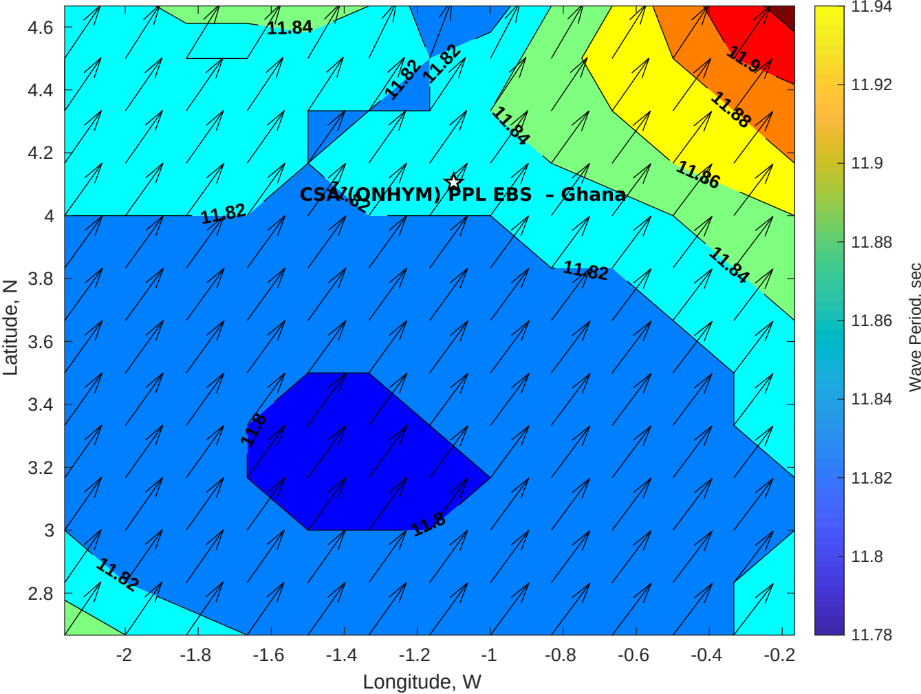
Wave Period (sec) for CSA (ONHYM) PPL EBS - Ghana at 06-Aug-2025 09:00:00
