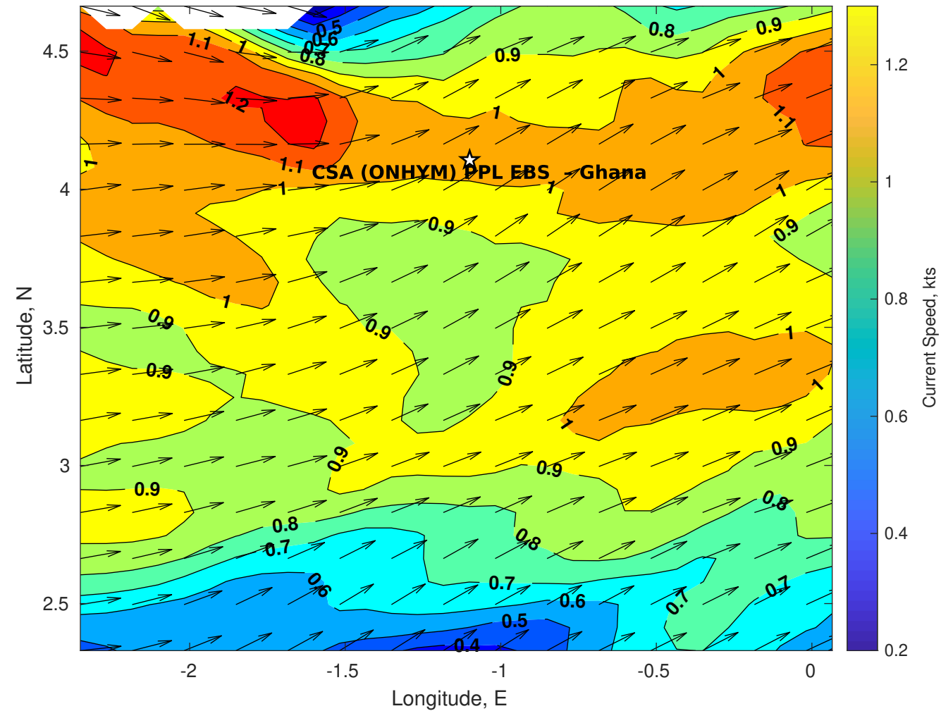
Surface Currents for CSA (ONHYM) PPL EBS - Ghana at 05-Aug-2025 00:00:00
