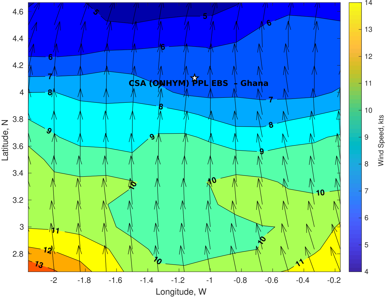
Winds (kts) for CSA (ONHYM) PPL EBS - Ghana at 06-Aug-2025 09:00:00
