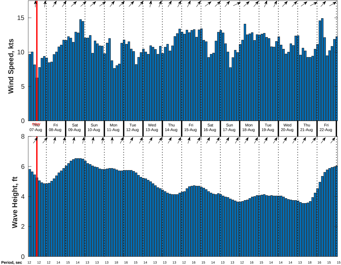
Wind & Wave Forecast for CSA (ONHYM) PPL EBS - Ghana from 06-Aug-2025 02:00:00 to 22-Aug-2025 02:00:00
