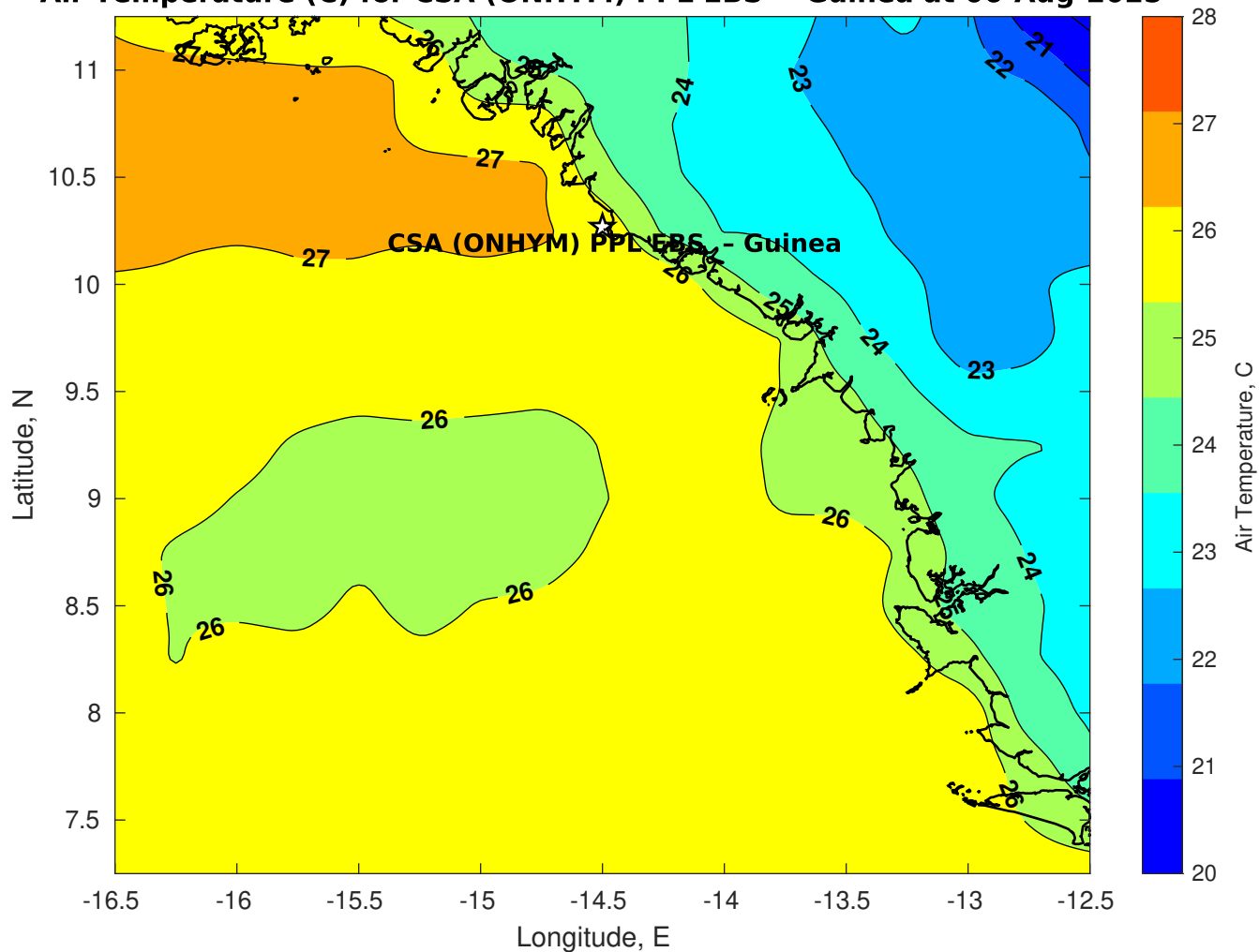
Air Temperature (C) for CSA (ONHYM) PPL EBS - Guinea at 06-Aug-2025
