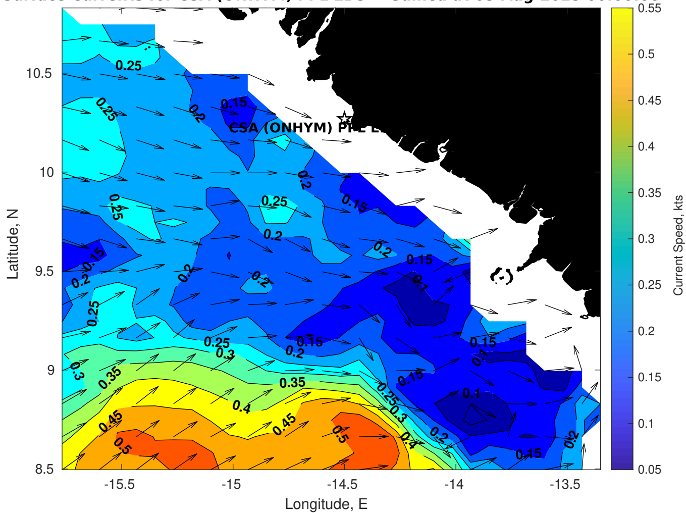
Surface Currents for CSA (ONHYM) PPL EBS - Guinea at 05-Aug-2025 00:00:00
