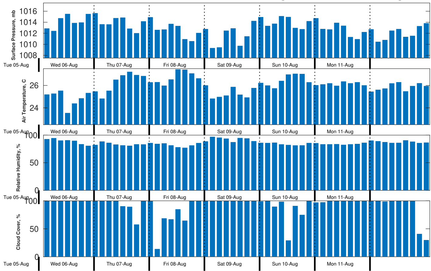
Met Forecast for CSA (ONHYM) PPL EBS - Guinea from 06-Aug-2025 00:00:00 to 13-Aug-2025 00:00:00
