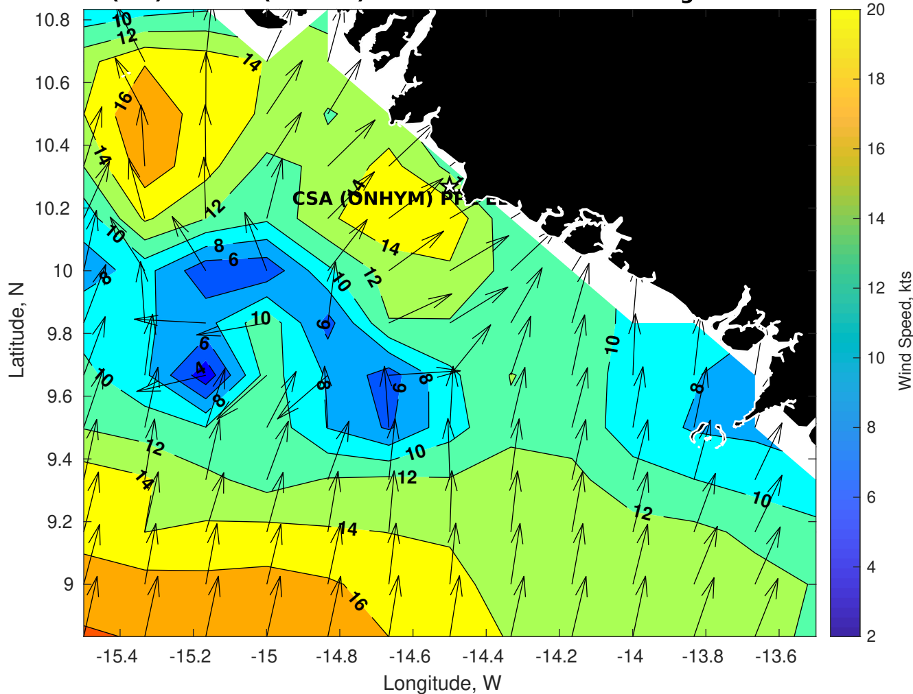
Winds (kts) for CSA (ONHYM) PPL EBS - Guinea at 06-Aug-2025 09:00:00
