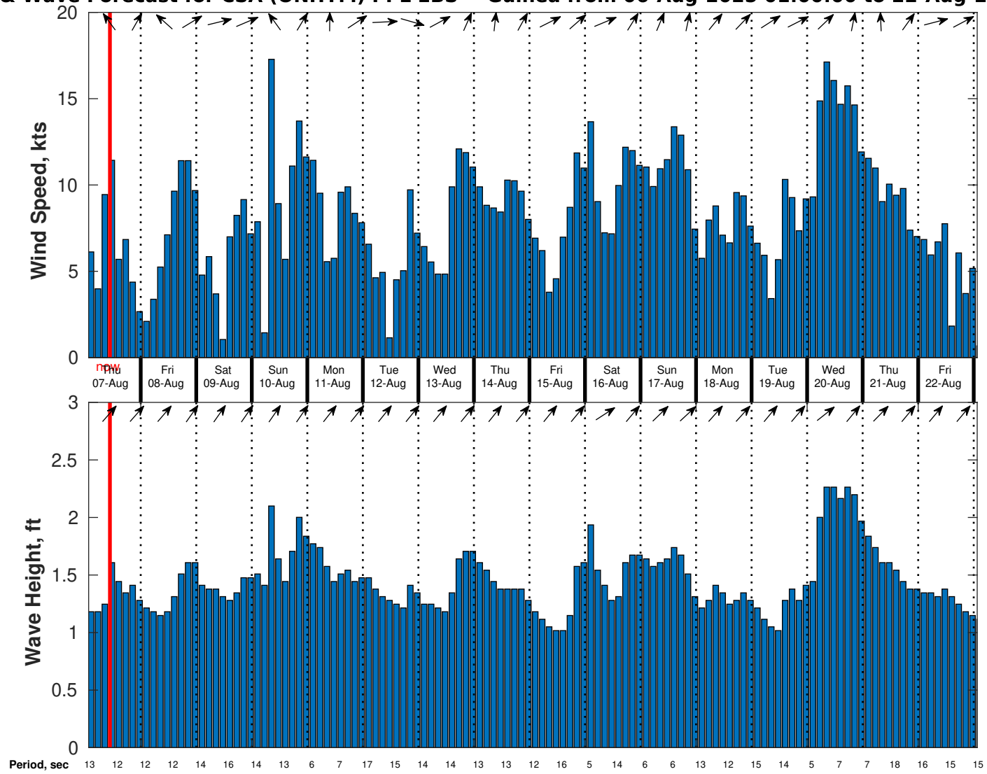
Wind & Wave Forecast for CSA (ONHYM) PPL EBS - Guinea from 06-Aug-2025 01:00:00 to 22-Aug-2025 01:00:00
