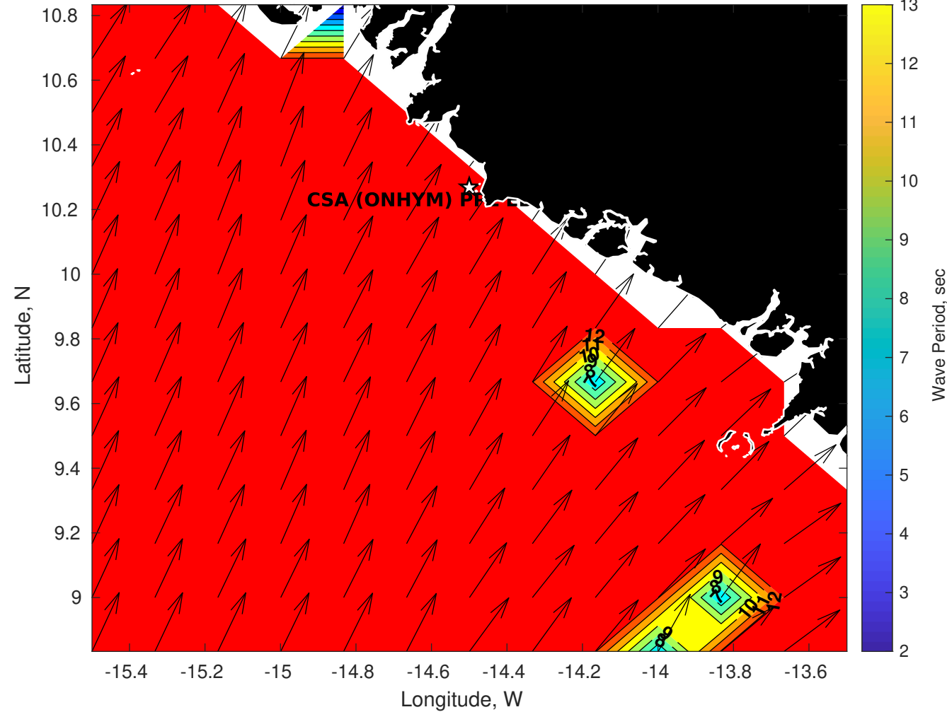
Wave Period (sec) for CSA (ONHYM) PPL EBS - Guinea at 06-Aug-2025 09:00:00
