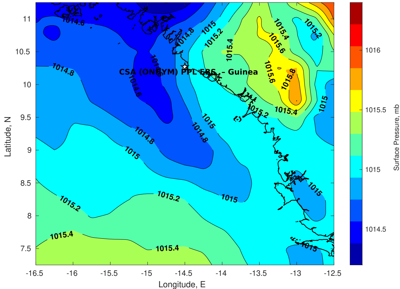
Surface Pressure (mb) for CSA (ONHYM) PPL EBS - Guinea at 08-Aug-2025 00:00:00
