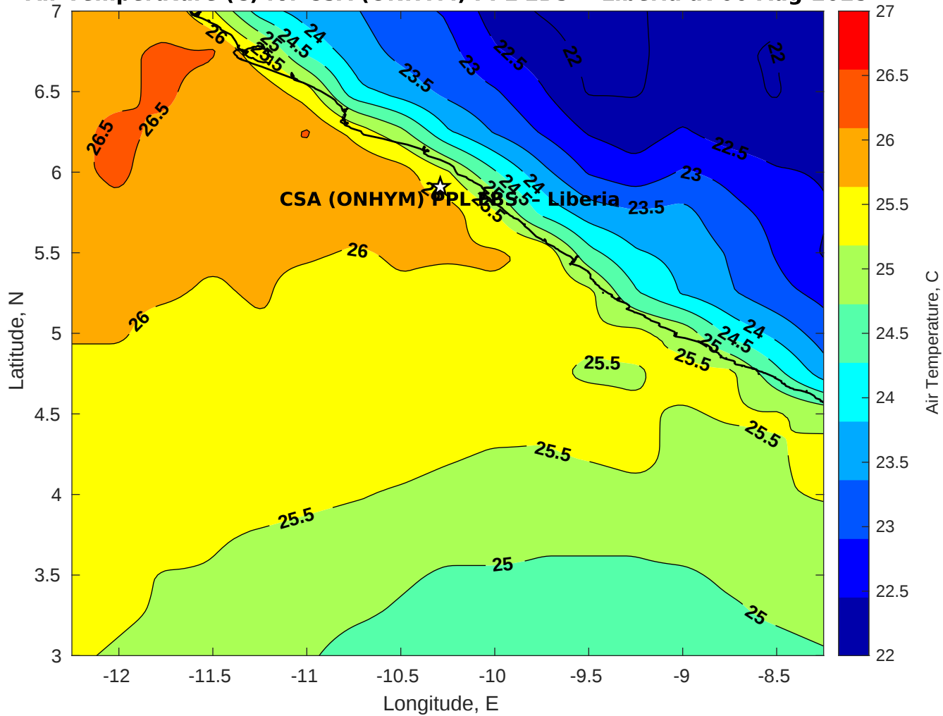
Air Temperature (C) for CSA (ONHYM) PPL EBS - Liberia at 06-Aug-2025
