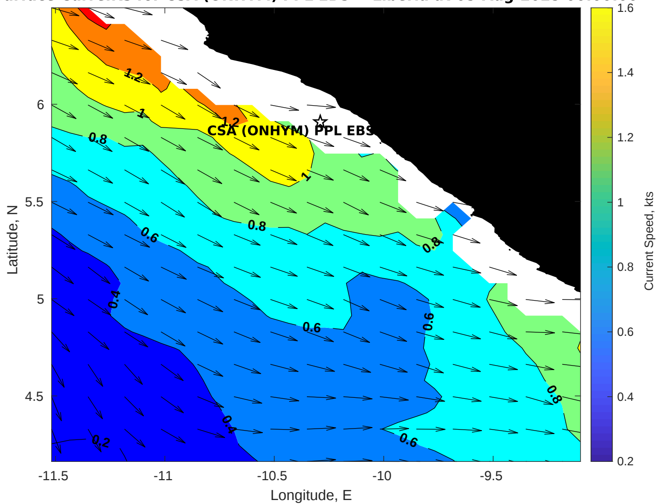
Surface Currents for CSA (ONHYM) PPL EBS - Liberia at 05-Aug-2025 00:00:00
