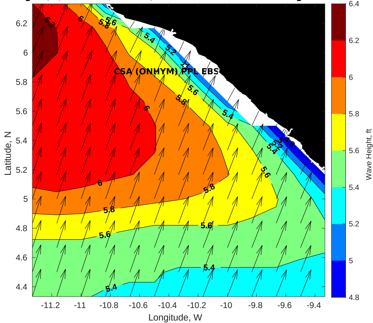
Wave Height (ft) for CSA (ONHYM) PPL EBS - Liberia at 06-Aug-2025 09:00:00
