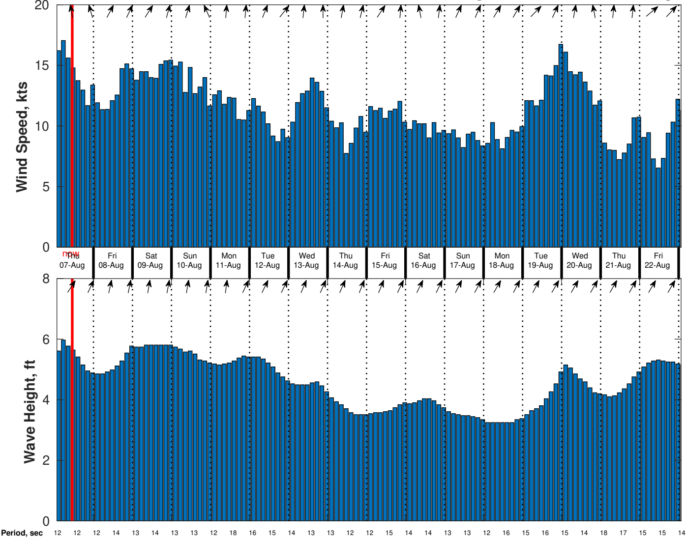
Wind & Wave Forecast for CSA (ONHYM) PPL EBS - Liberia from 06-Aug-2025 01:00:00 to 22-Aug-2025 01:00:00
