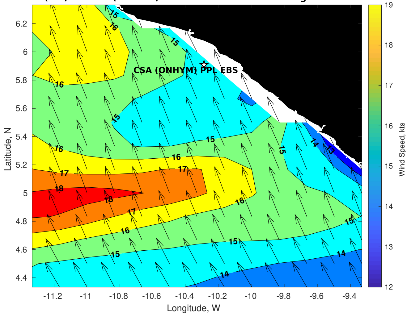
Winds (kts) for CSA (ONHYM) PPL EBS - Liberia at 06-Aug-2025 09:00:00
