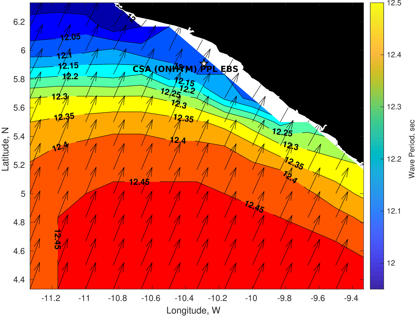
Wave Period (sec) for CSA (ONHYM) PPL EBS - Liberia at 06-Aug-2025 09:00:00
