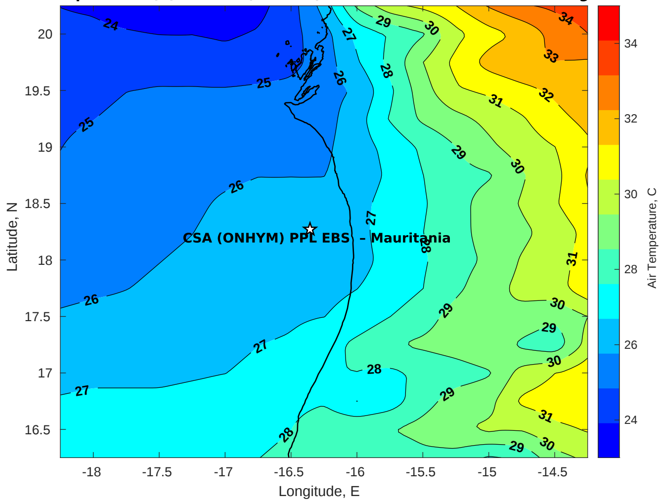
Air Temperature (C) for CSA (ONHYM) PPL EBS - Mauritania at 06-Aug-2025
