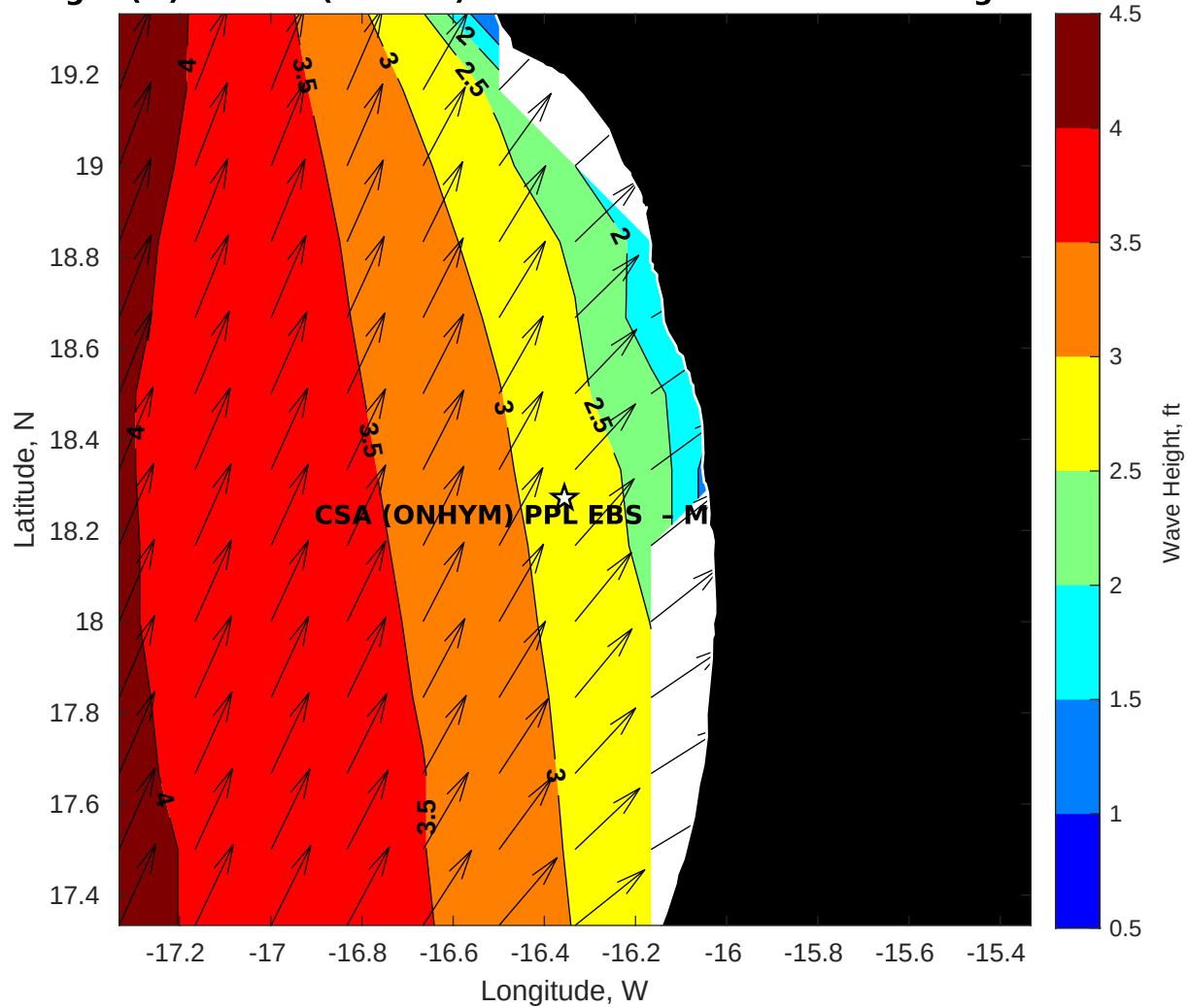
Wave Height (ft) for CSA (ONHYM) PPL EBS - Mauritania at 06-Aug-2025 09:00:00
