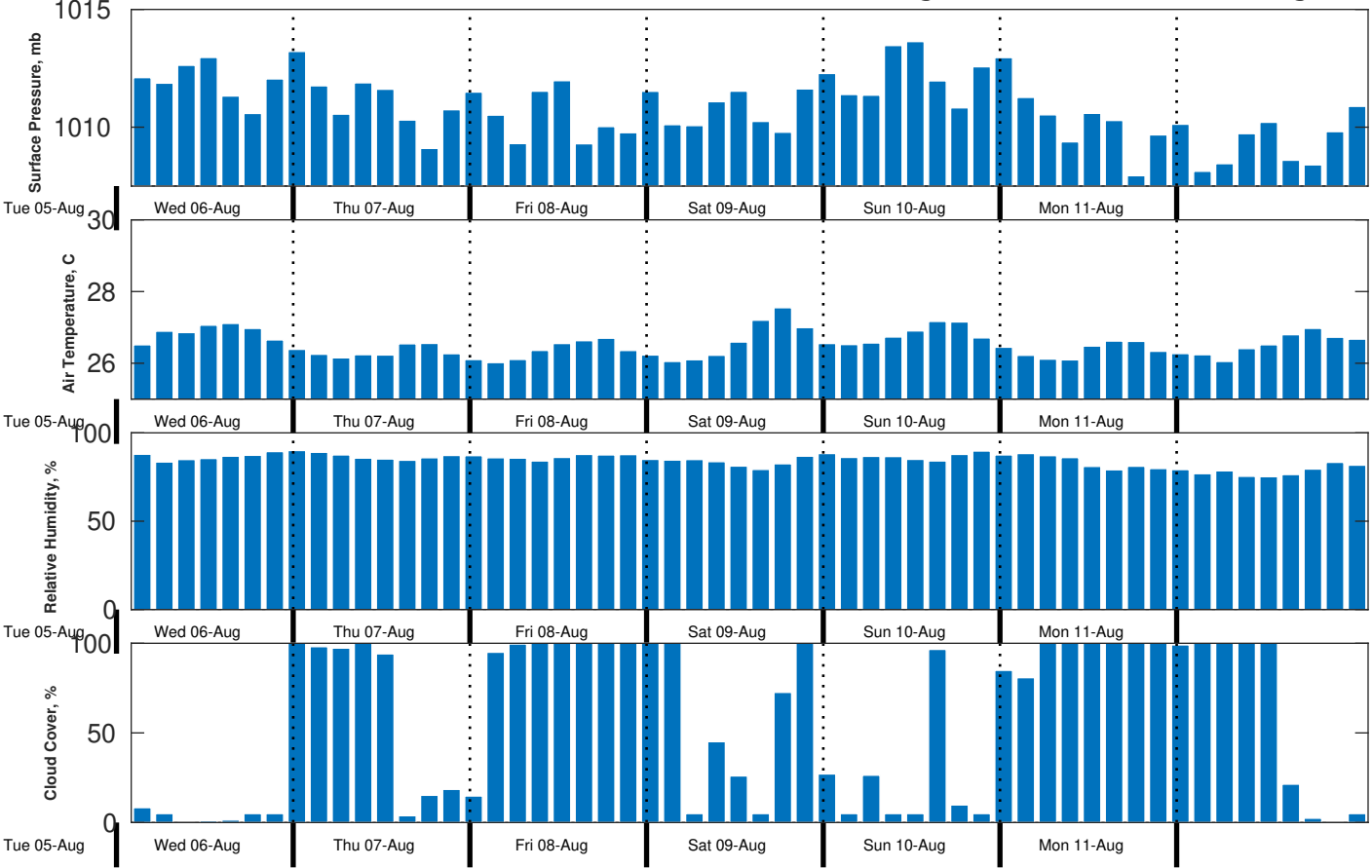
Met Forecast for CSA (ONHYM) PPL EBS - Mauritania from 06-Aug-2025 00:00:00 to 13-Aug-2025 00:00:00
