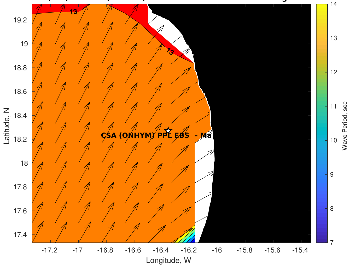
Wave Period (sec) for CSA (ONHYM) PPL EBS - Mauritania at 06-Aug-2025 09:00:00
