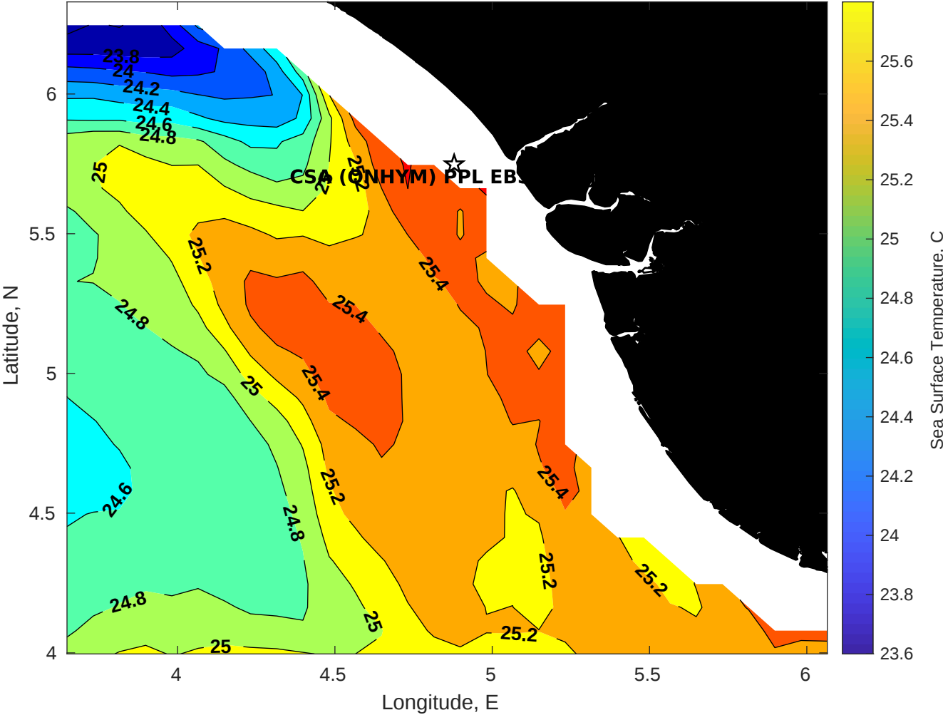
SST for CSA (ONHYM) PPL EBS - Nigeria at 05-Aug-2025 00:00:00
