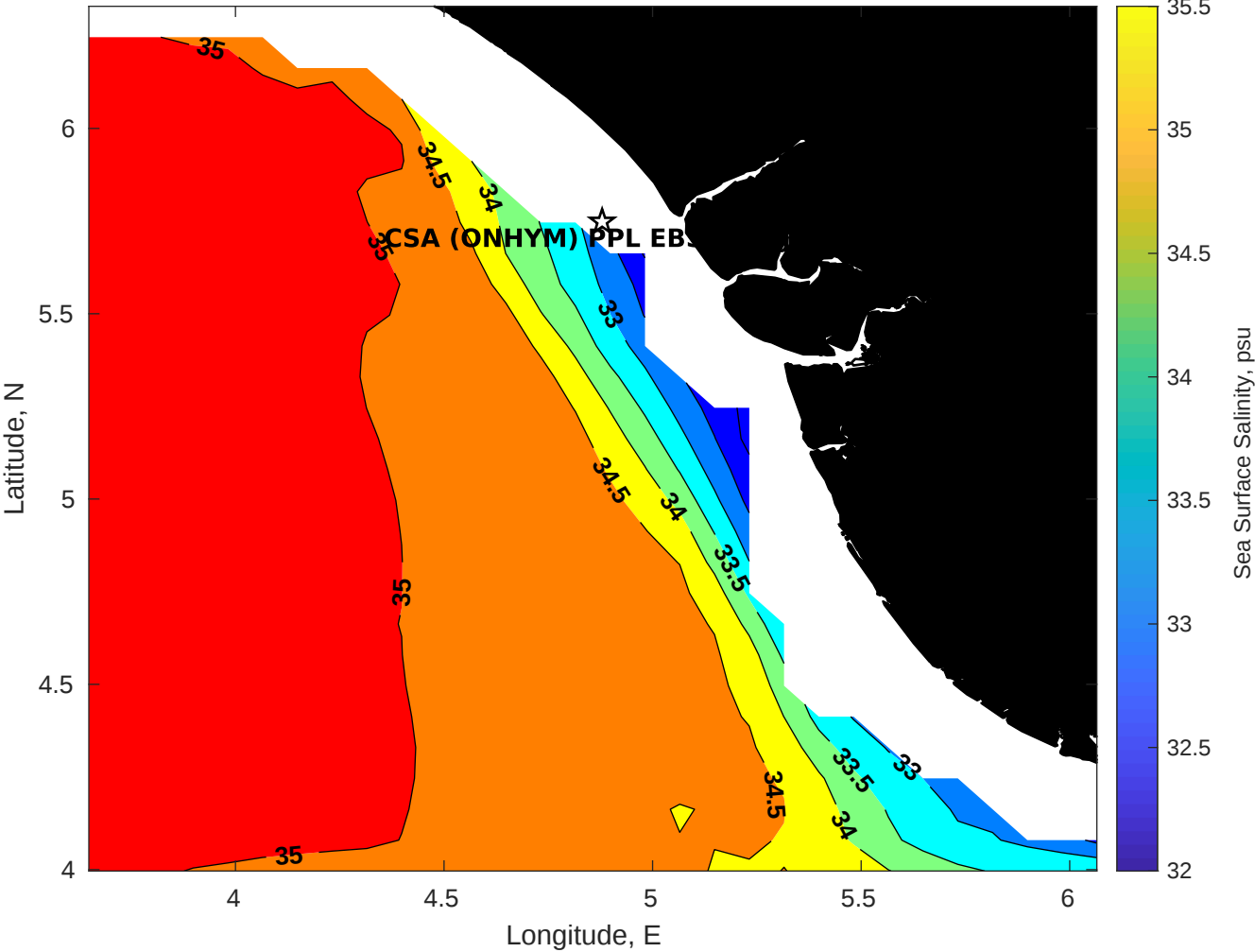
Surface Salinity for CSA (ONHYM) PPL EBS - Nigeria at 05-Aug-2025 00:00:00
