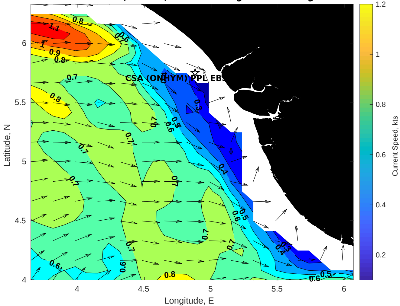
Surface Currents for CSA (ONHYM) PPL EBS - Nigeria at 05-Aug-2025 00:00:00
