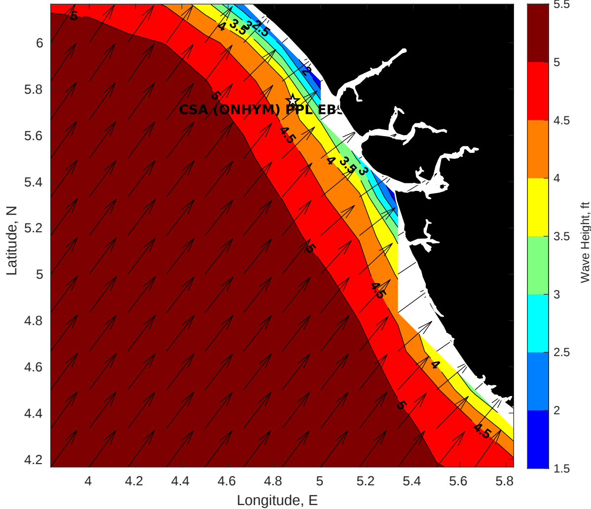
Wave Height (ft) for CSA (ONHYM) PPL EBS - Nigeria at 06-Aug-2025 09:00:00
