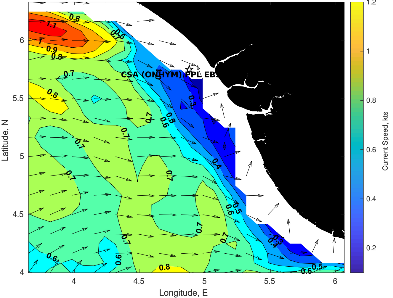
Surface Currents for CSA (ONHYM) PPL EBS - Nigeria at 05-Aug-2025 00:00:00
