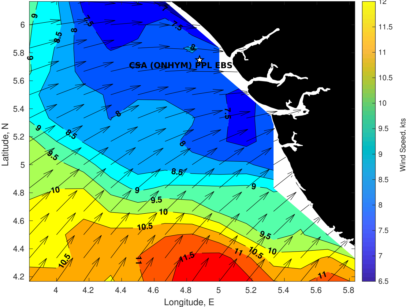
Winds (kts) for CSA (ONHYM) PPL EBS - Nigeria at 06-Aug-2025 09:00:00
