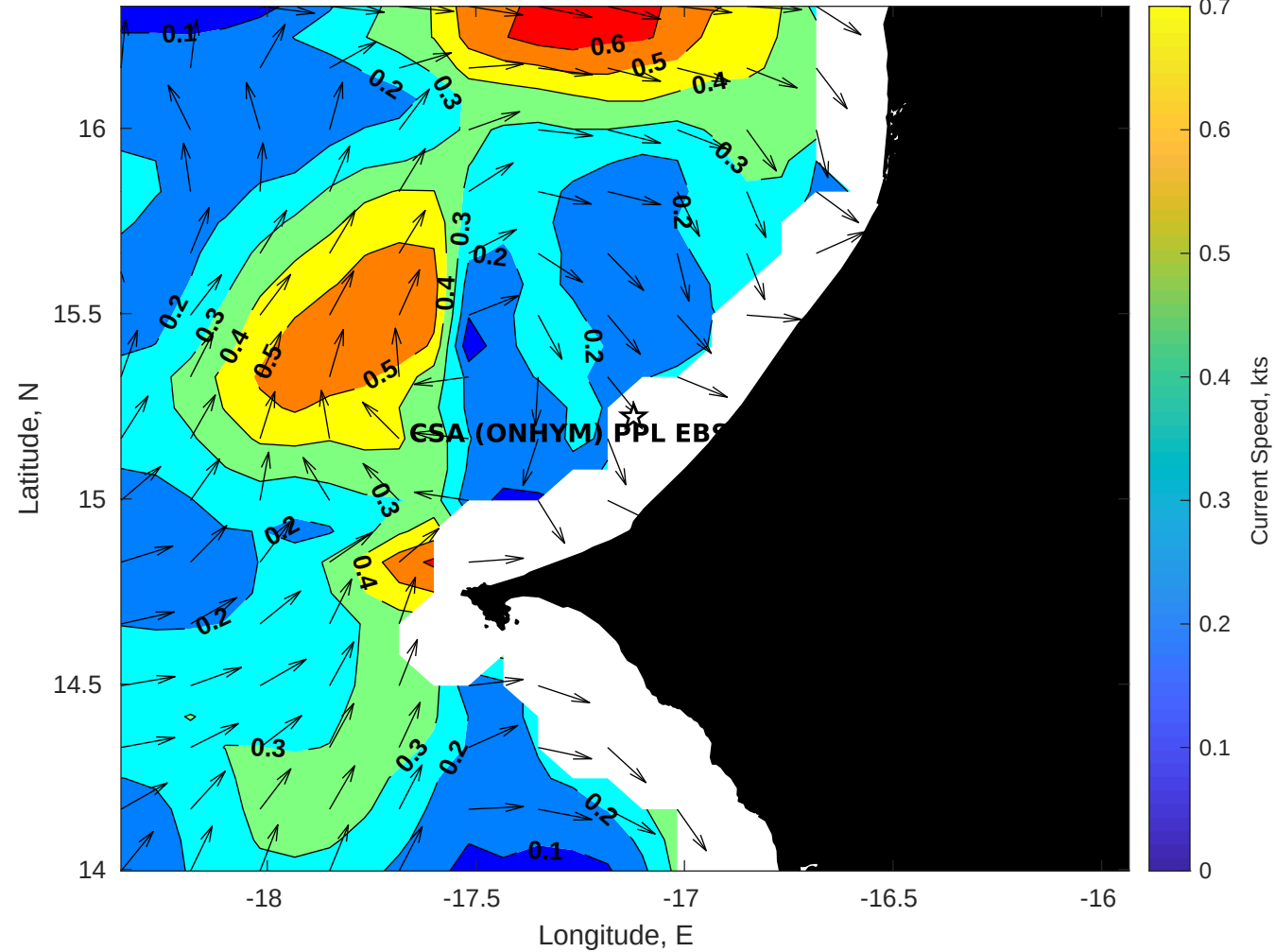
Surface Currents for CSA (ONHYM) PPL EBS - Senegal at 05-Aug-2025 00:00:00
