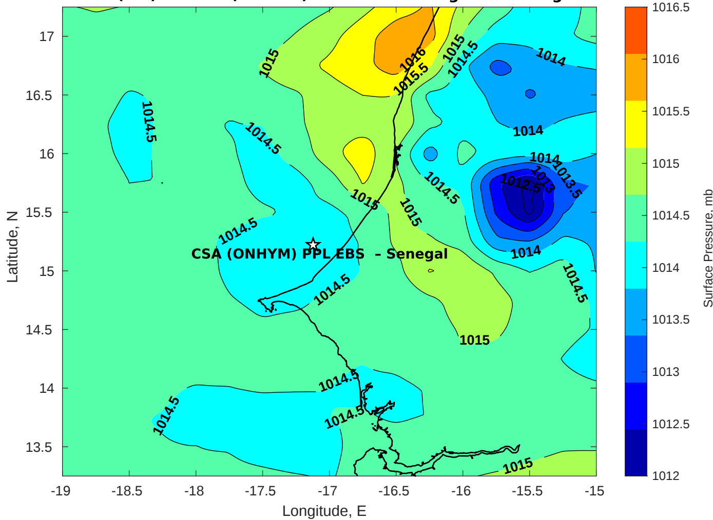
Surface Pressure (mb) for CSA (ONHYM) PPL EBS - Senegal at 07-Aug-2025 00:00:00
