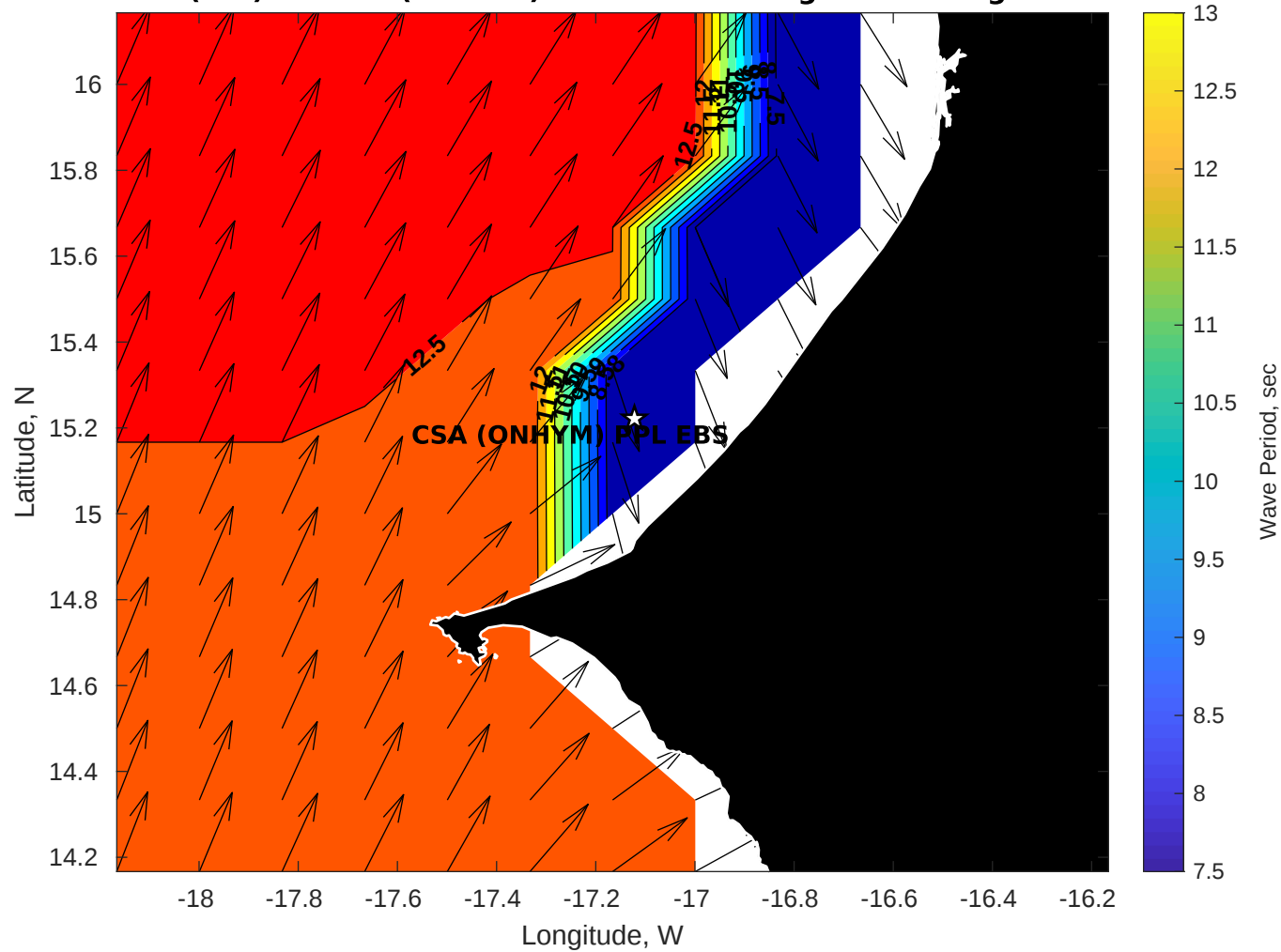
Wave Period (sec) for CSA (ONHYM) PPL EBS - Senegal at 06-Aug-2025 09:00:00
