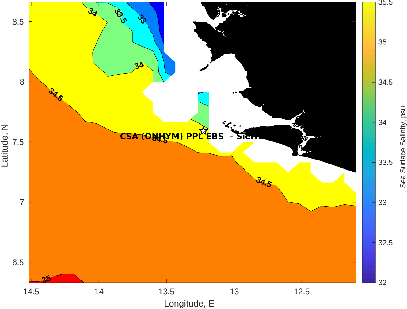
Surface Salinity for CSA (ONHYM) PPL EBS - Sierra Leone at 05-Aug-2025 00:00:00
